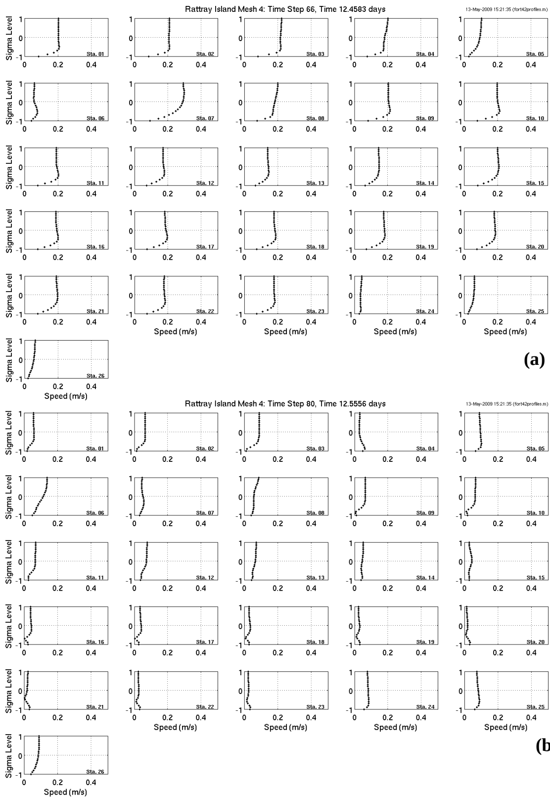
Figure 6.6 Vertical profiles of the modeled currents at each of the 26 current meter locations on 28 November 1982, (a) 11hrs and (b) 13.3hrs.
