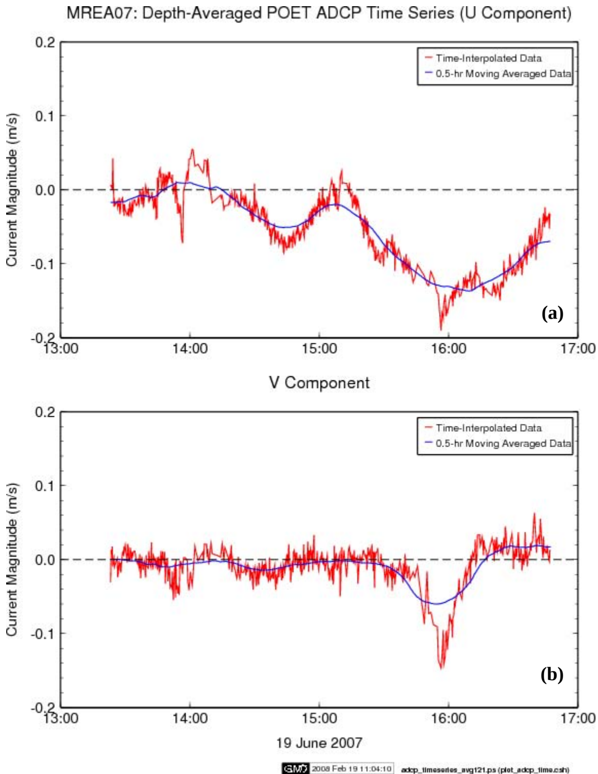
Figure 7.10. Time-interpolated (a) U and (b) V components of the current observations (red) and the \frac{1}{2} hour moving averaged data (blue).
