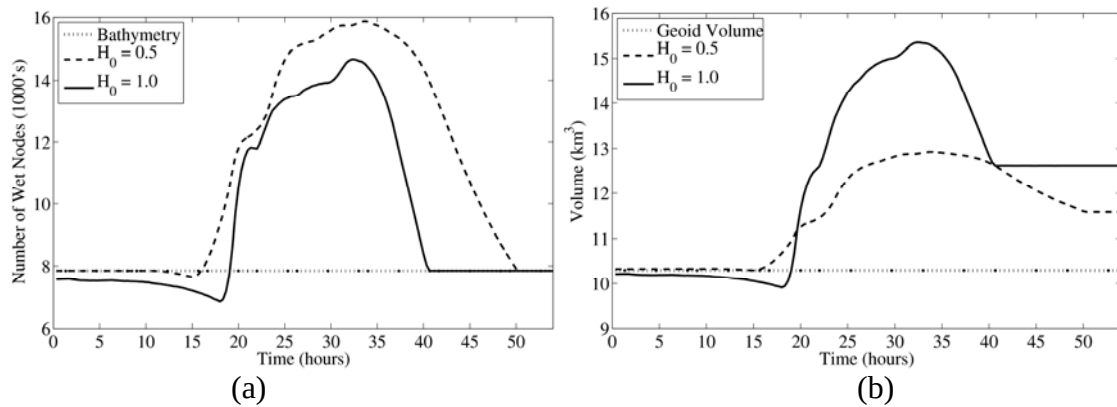
Figure 2.5. In (a) the number of wet nodes and in (b) the computed total volume of water during the simulation for two H_o values, H_o = 0.5 and H_o = 1.0 , with V_{min} = 0.05 .
