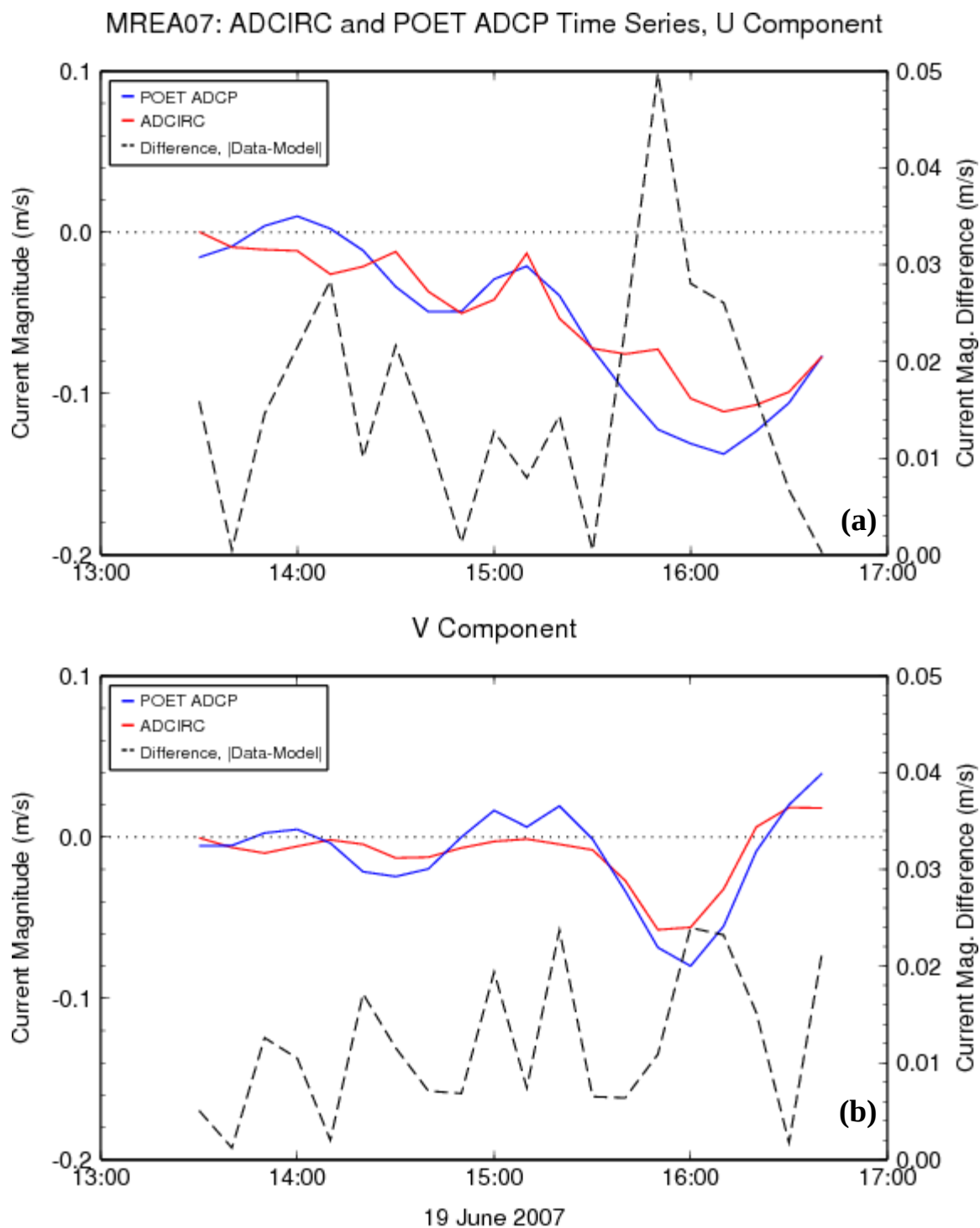
Figure 7.11. Modeled (red) and observed (a) U and (b) V components of the current; the difference is shown in black (right-hand scale).
