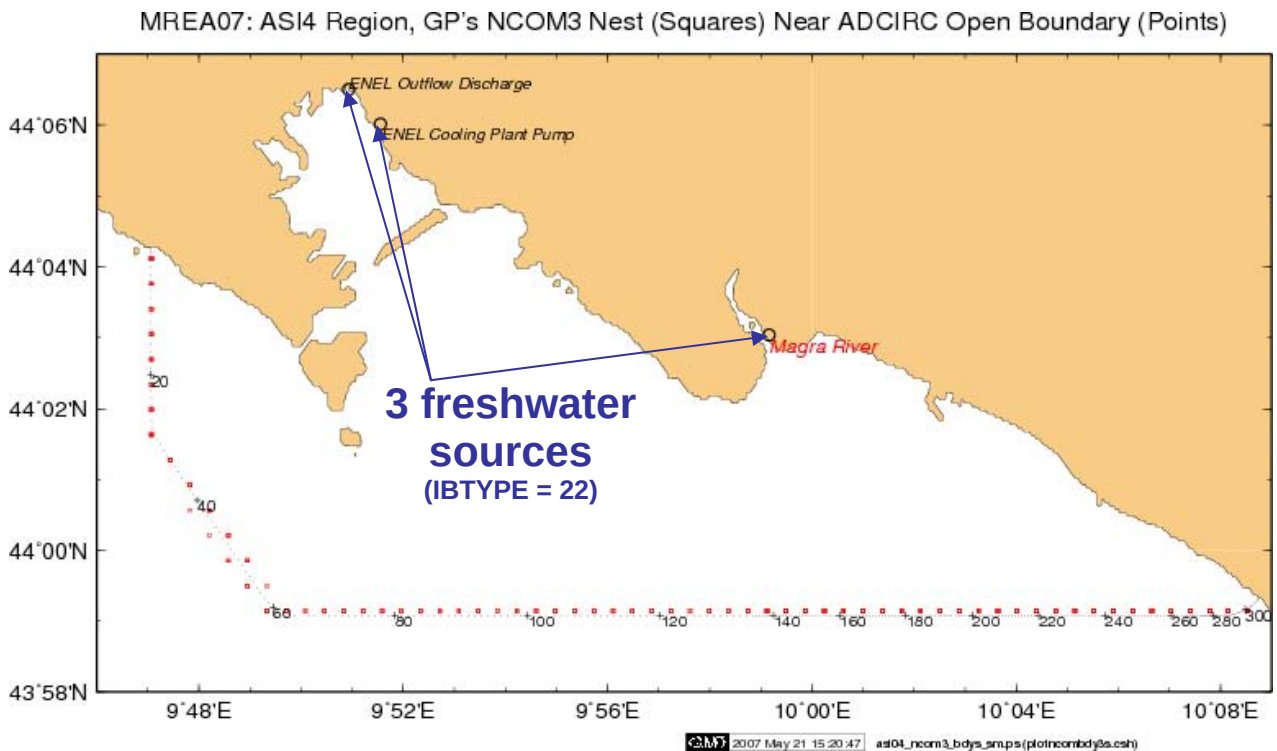
Figure 7.4. Freshwater discharge locations of the ENEL Outflow, the ENEL Cooling Plant Pump, and the Magra River. The ENEL daily discharges are each specified as 30 \text{ m}^3/\text{s} .
