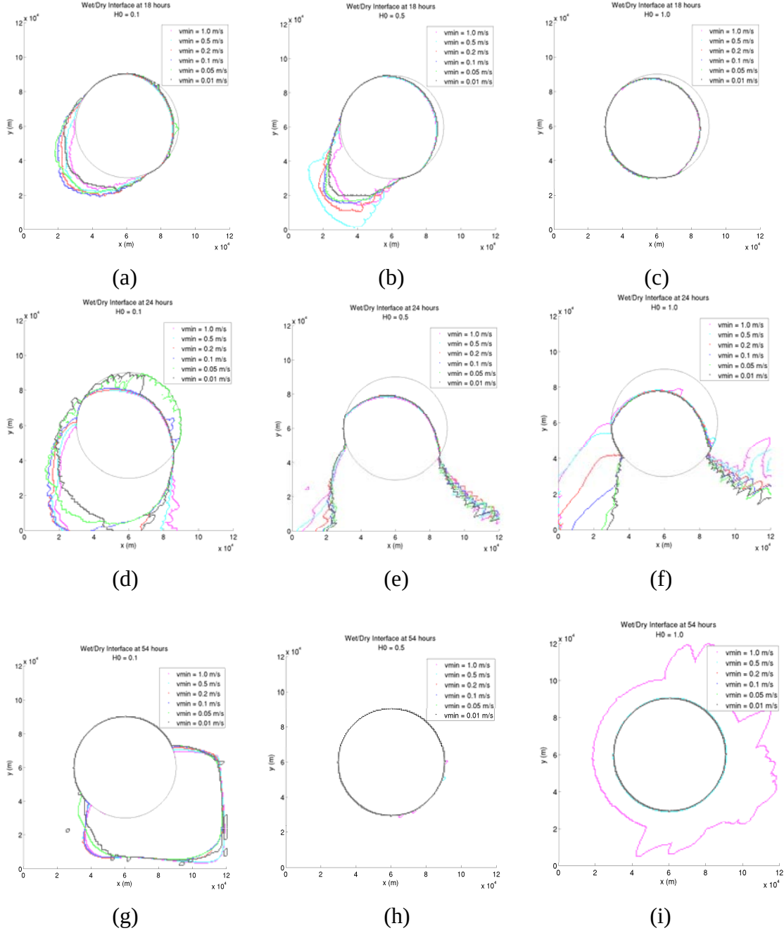
Figure 2.3. Contours of the wetting and drying front at 18, 24 and 54 hours (rows) into the simulation, using different H_0 values (columns), and different V_{min} values represented by different color contours lines. The original coastline of the basin (in black) is included as a frame of reference.
