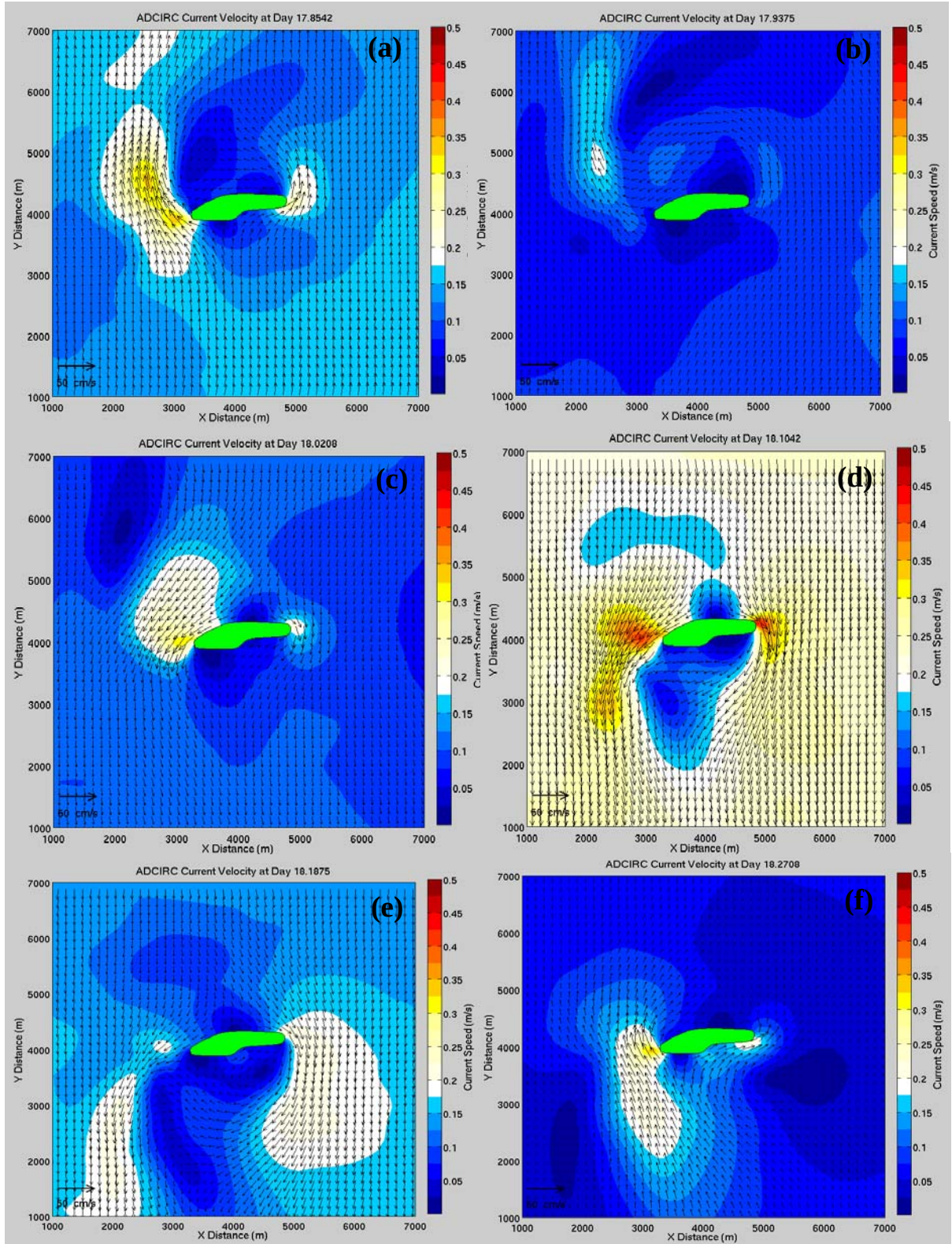
Figure 6.8: Computed currents on 04 December 1982 at (a) 3.6 hrs, (b) 5.6 hrs, (c) 7.6 hrs, (d) 9.6 hrs, (e) 11.6hrs, and (f) 13.6hrs.
