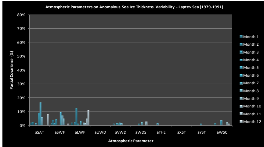
Figure 85. Anomalous Sea Ice Thickness Variability—Laptev Sea (1979-1991)
