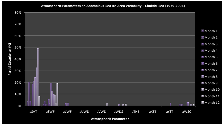
Figure 71. Anomalous Sea Ice Area Variability—Chukchi Sea (1979-2004)
