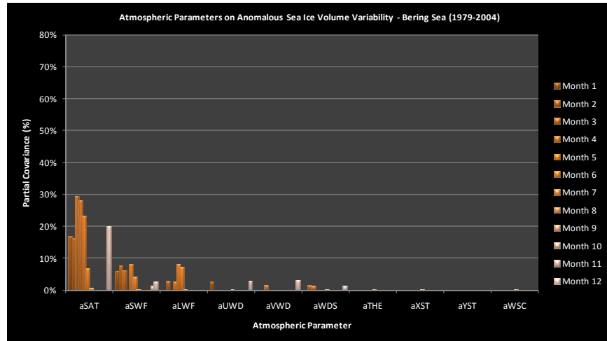
Figure 147. Anomalous Sea Ice Volume Variability—Bering Sea (1979-2004) (same as Figure 41)
