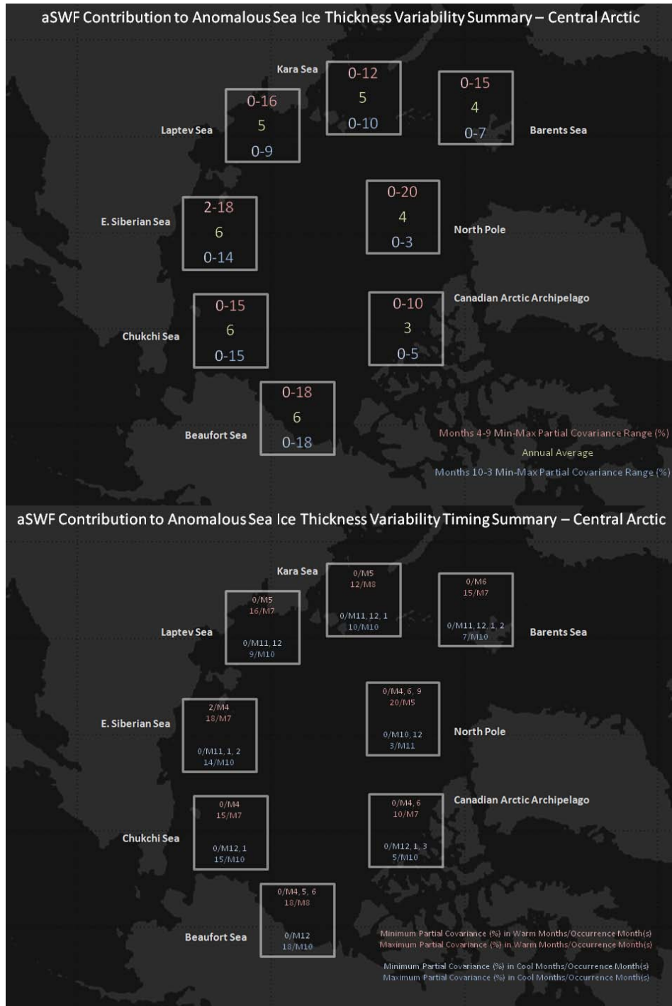
Figure 178. (Top) Average (green), Warming Months Minimum-Maximum Range (red), and Cooling Months Minimum-Maximum Range (blue) of aSWF Contribution to aTHKv (top) and Timing of Warming (red) and Cooling (blue) Minimum and Maximum (bottom)—Central Arctic (1979–2004)
