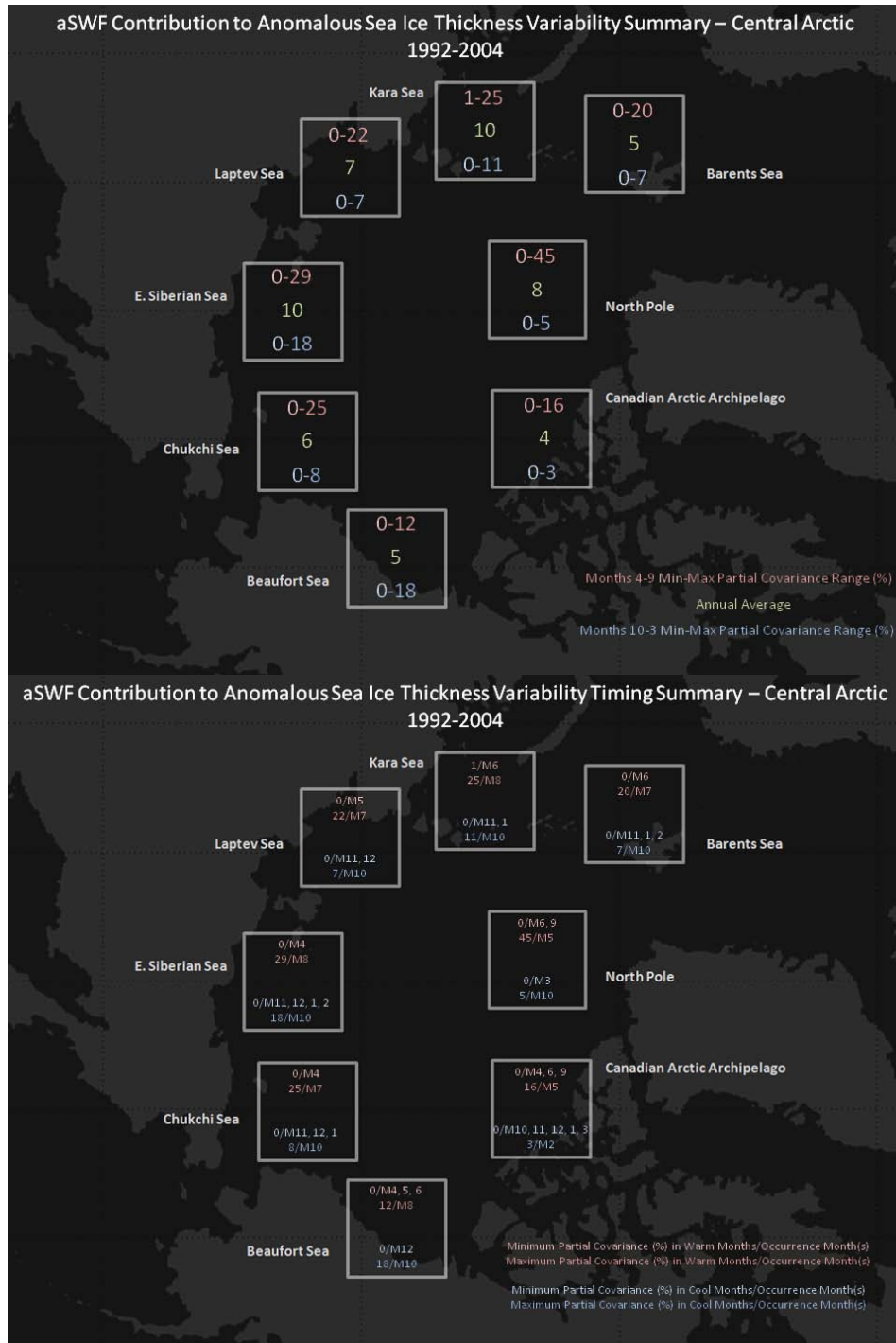
Figure 184. Average (green), Warming Months Minimum-Maximum Range (red), and Cooling Months Minimum-Maximum Range (blue) of aSWF Contribution to aTHKv (top) and Timing of Warming (red) and Cooling (blue) Minimum and Maximum (bottom)—Central Arctic (1992–2004)
