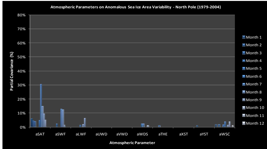
Figure 73. Anomalous Sea Ice Area Variability—North Pole (1979-2004)
