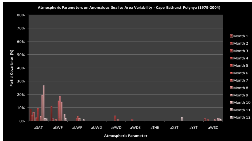
Figure 40. Anomalous Sea Ice Area Variability—Cape Bathurst Polynya (1979–2004)
