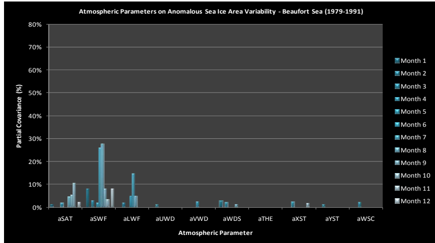
Figure 96. Anomalous Sea Ice Area Variability—Beaufort Sea (1979-1991)
