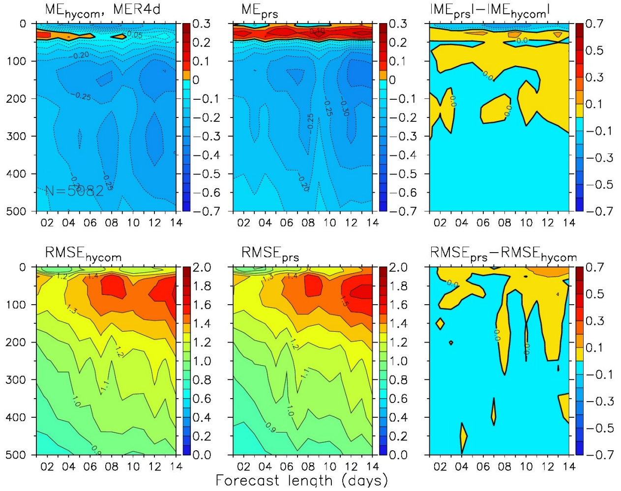
Figure 21: As in Figure 20 except for region MER4d. The average number of profiles used on each forecast day is 5082.
