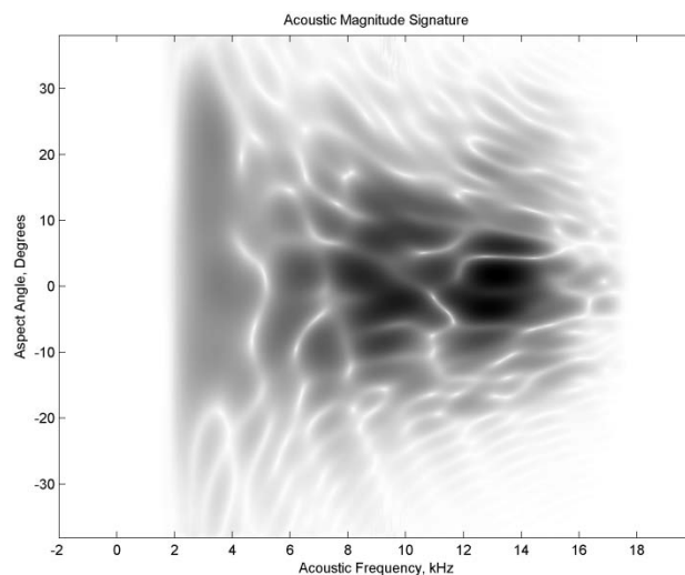
Figure 9 is the acoustic magnitude signature for the metallic sphere.
