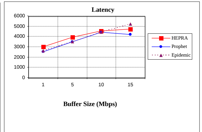
Figure 6. HEPRA reduces latency when size of buffer increases
