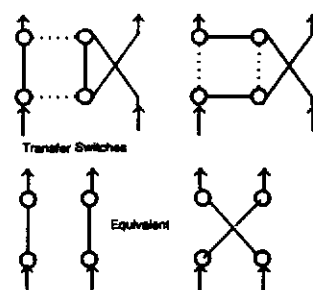
Figure 9. Transfer Switches
