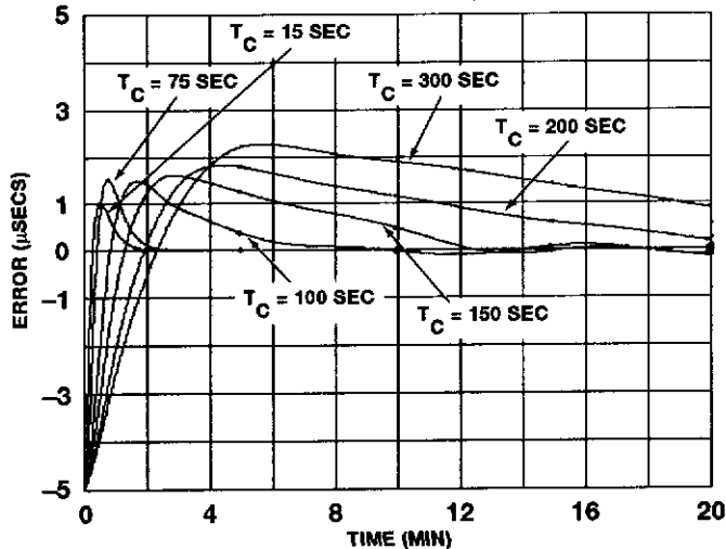
Figure 9: Loop Transient Response When Using RAFS (Variation With Loop Time Constant)
