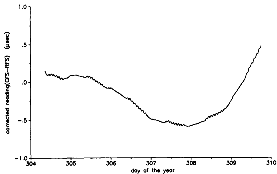
Figure 1 Reading(RFS-CFS), temperature corrected
