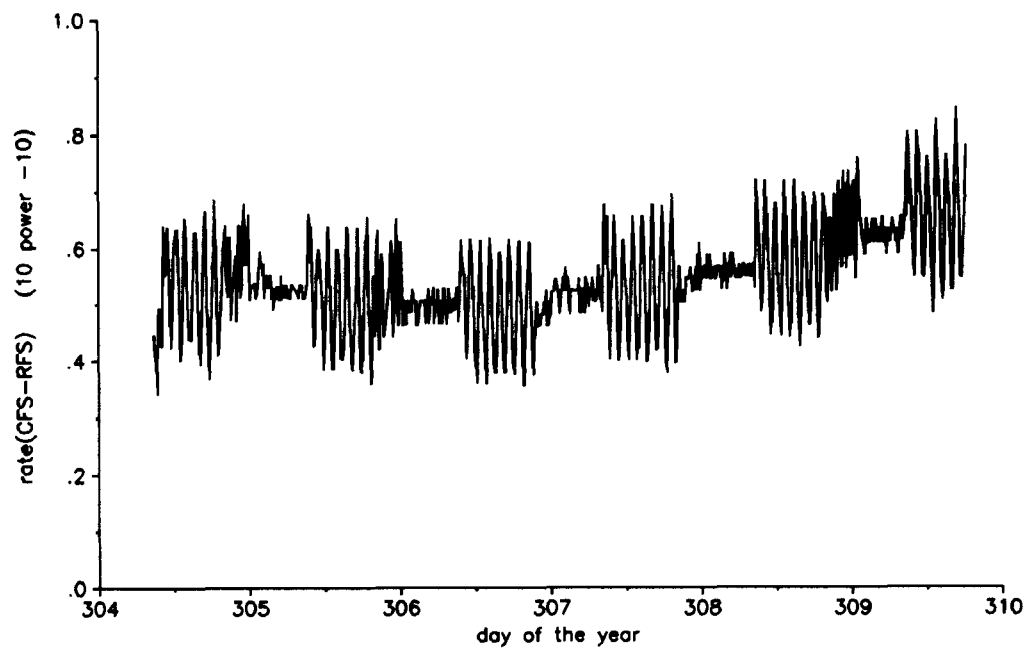
Figure 4 Rate(RFS-CFS), best temperature correction Shuttle attitude (above)
