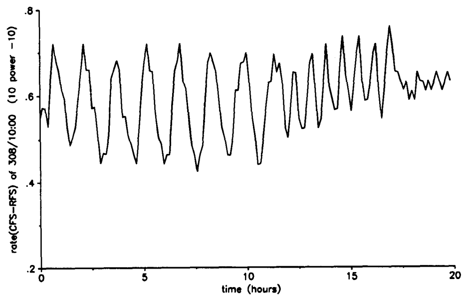
Figure 2 Rate(RFS-CFS), best temperature correction, time slice of 20 hours
