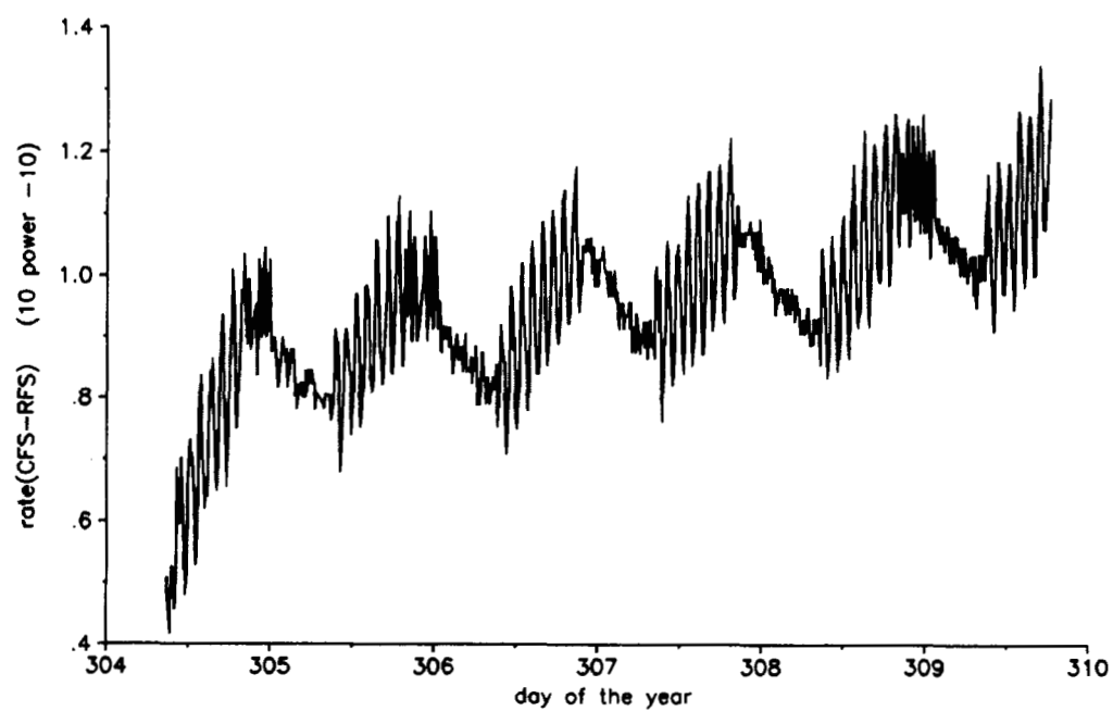
Figure 3 Rate(RFS-CFS), corrected by ground temperature coefficient Temperature curve (above)
