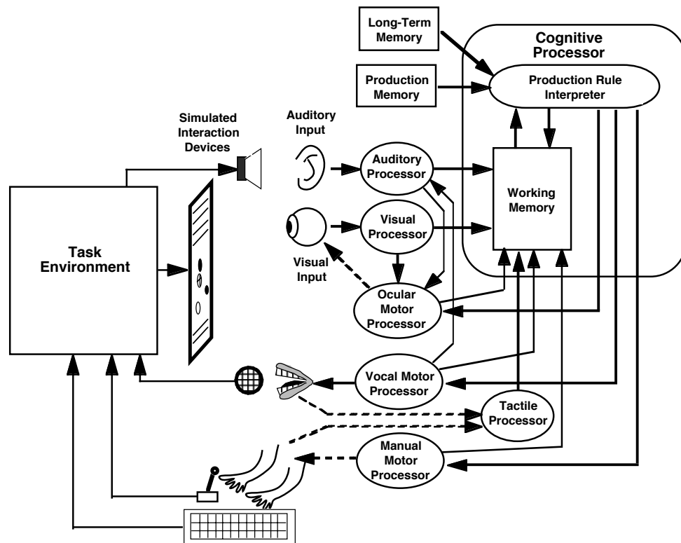
Figure 1. The high-level architecture of the EPIC cognitive architecture (Kieras & Meyer, 1997).
