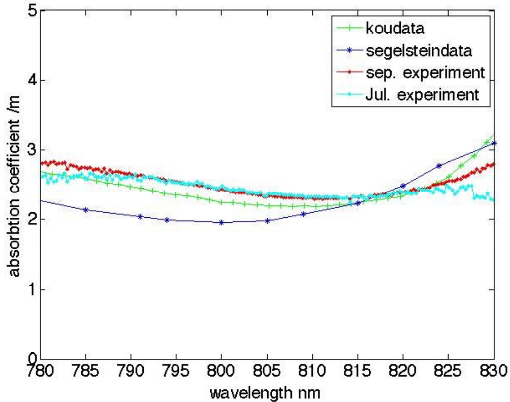
Fig. 6. Comparison of our absorption coefficient determination using ultrashort pulses with that of both Kou 28 , et. al. and Segelstein 29 . Note the better agreement with Kou's data.
