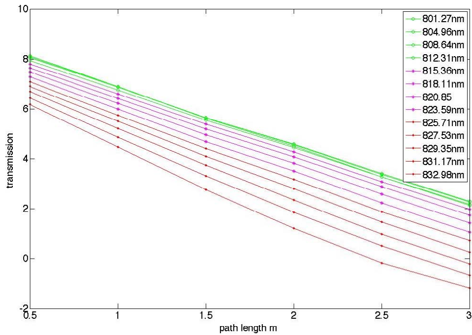
Fig. 5. Separate frequencies from the pulse above as a function of distance. Note the BLB behavior of each frequency
