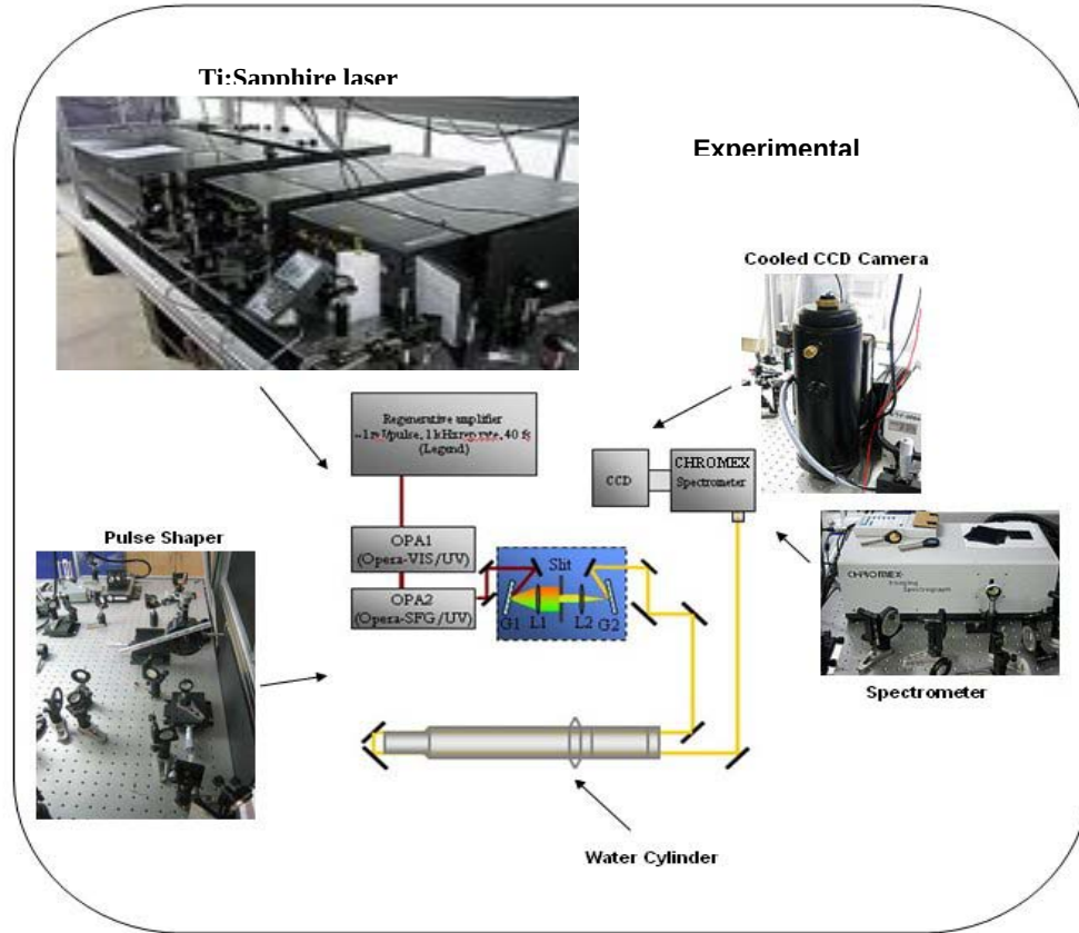
Fig. 3. Experimental setup schematics.
