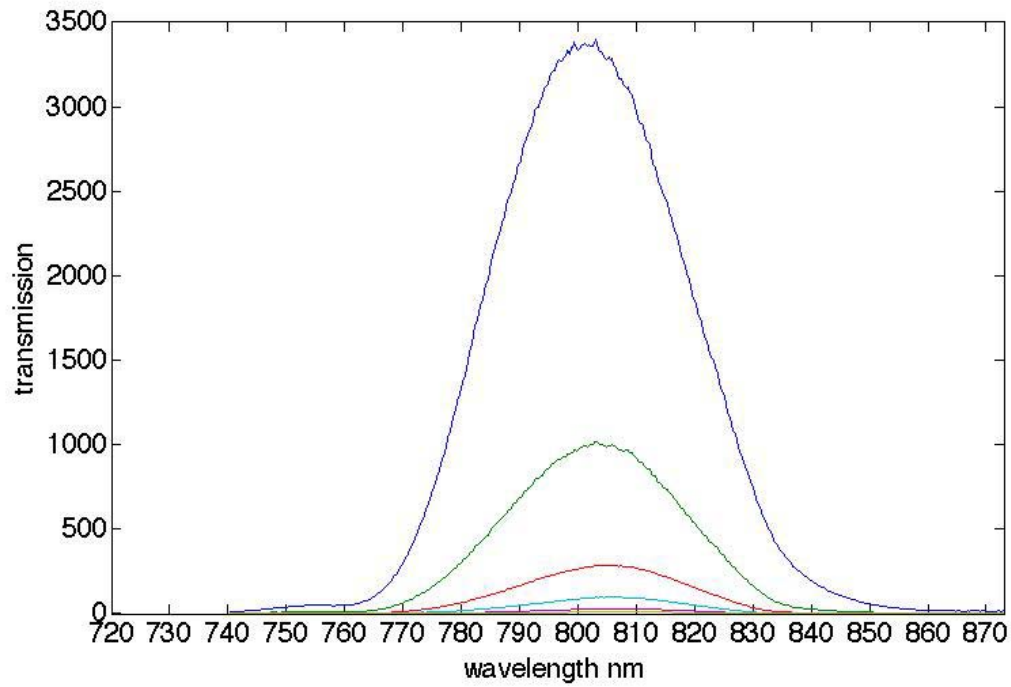
Fig. 4. Pulse shape as a function of distance of propagation in deionized water. The distances from top to bottom are z=0.5, 1, 1.5, 2, 2.5, and 3\text{m} .
