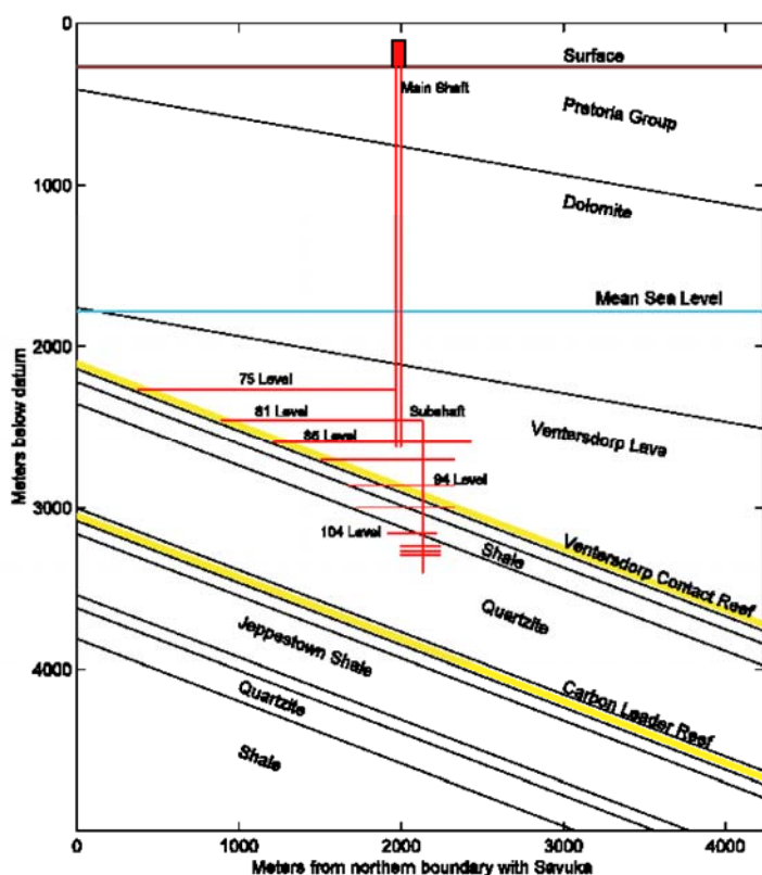
Figure 2. Cross-section through the main shaft of the Mponeng mine looking east. The two gold-bearing horizons are marked in yellow. The datum is measured from an elevation in Johannesburg, and so it is above the ground surface.
