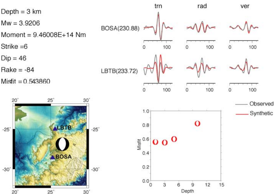
Figure 3. Body and surface waves from regional or near regional events were used to estimate the best fitting double-couple moment tensor. The technique minimizes the misfit between reflectivity generated complete synthetic seismograms and the three-component displacement data via a search over the strike, dip and rake of the source. An initial coarse grid-search to find the approximate minima is followed by a finer grid-search. For this event, we fitted the data over the period range of 20–50 sec. The displacements due to the six fundamental couples were calculated using Bowers (1997) velocity model. The best fit is obtained at 3-km depth.
