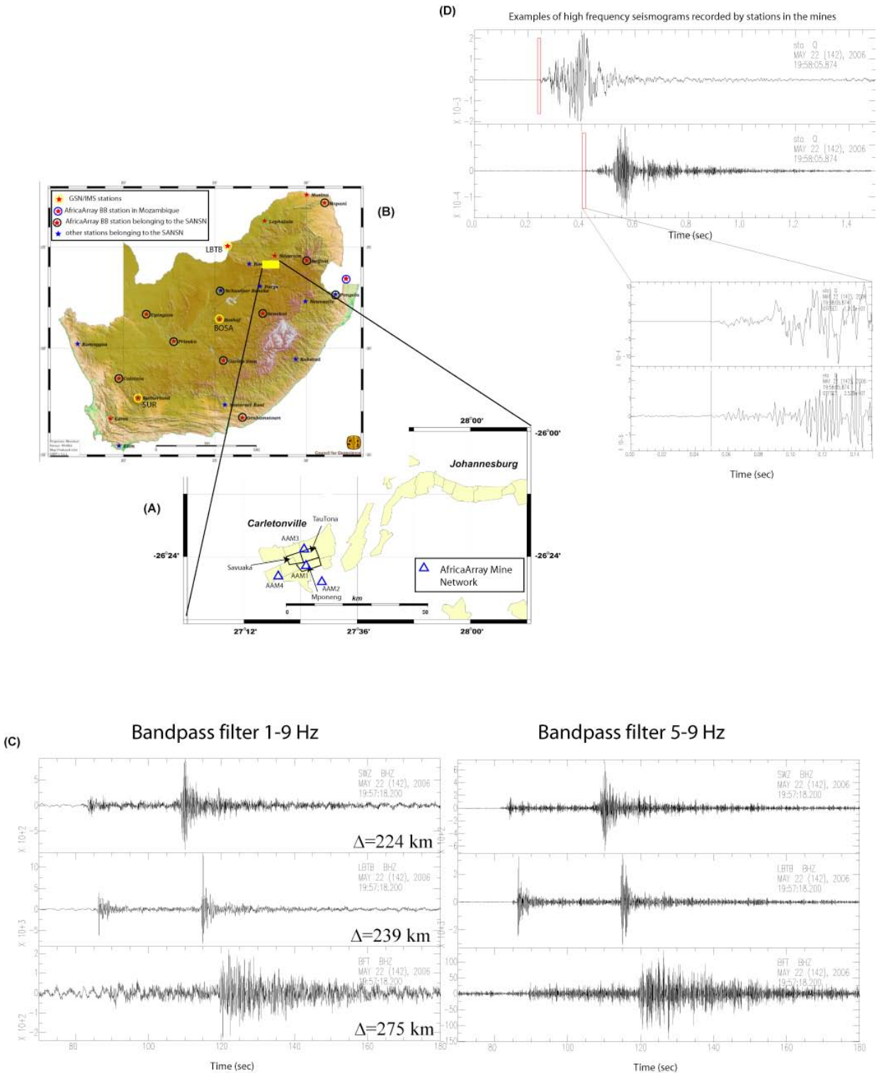
Figure 1. (a) Map showing the locations of the gold mines (yellow areas) on the northwestern side of the Witwatersrand basin (Far West Rand region). Data for this project come from the three mines labeled. The blue triangles show station locations of the surface mine network that has been constructed. (b) Map showing location of AfricaArray broadband stations at local and regional distances. (c) Vertical displacement seismograms from a M = 2.2 mining event recorded at near-regional distances. (d) The same event recorded on high-frequency in-mine seismic stations.
