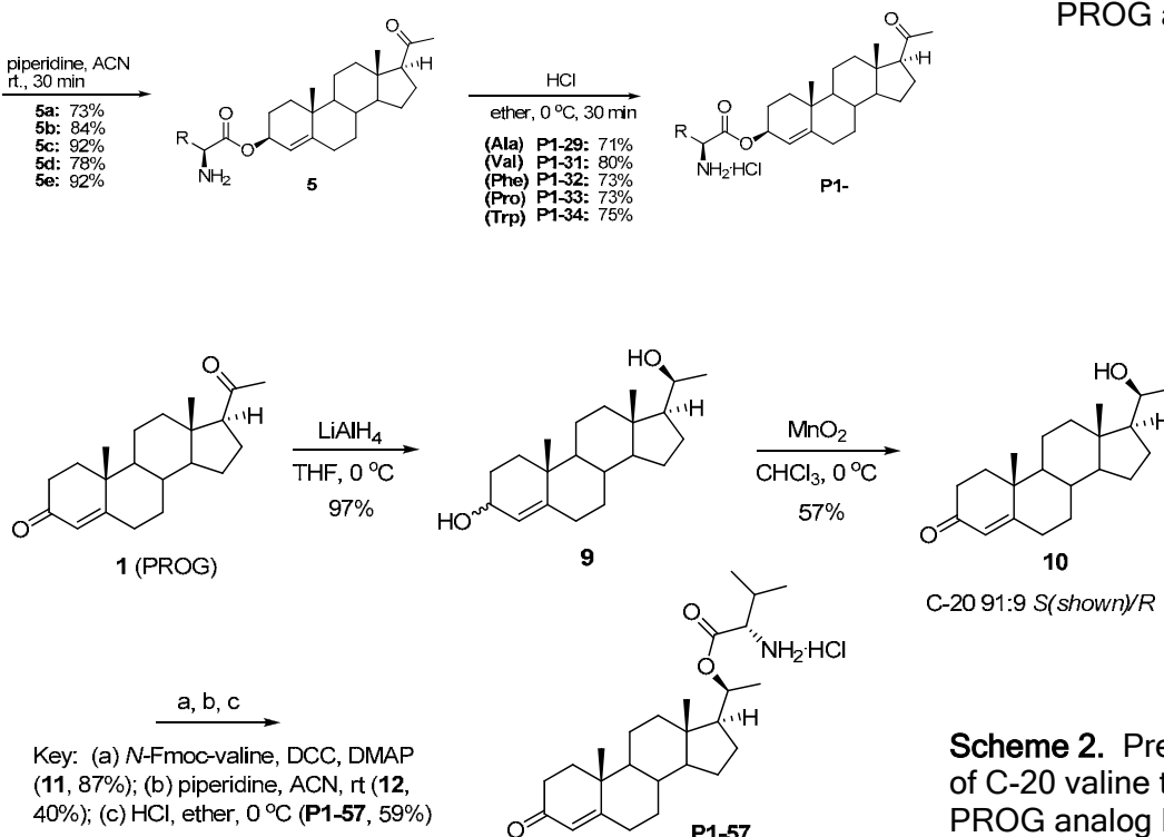
Scheme 1. Preparation of C-3 amino acid tethered PROG analogs.
