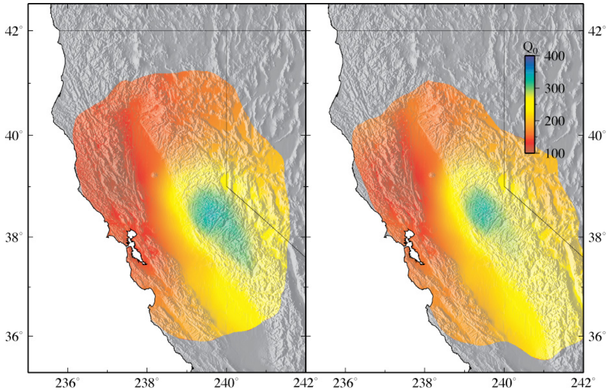
Figure 5. Attenuation tomography using amplitudes (a) where the source and site term is solved for in the inversion and (b) where the source term is removed from the amplitudes using a coda-derived moment rate.
