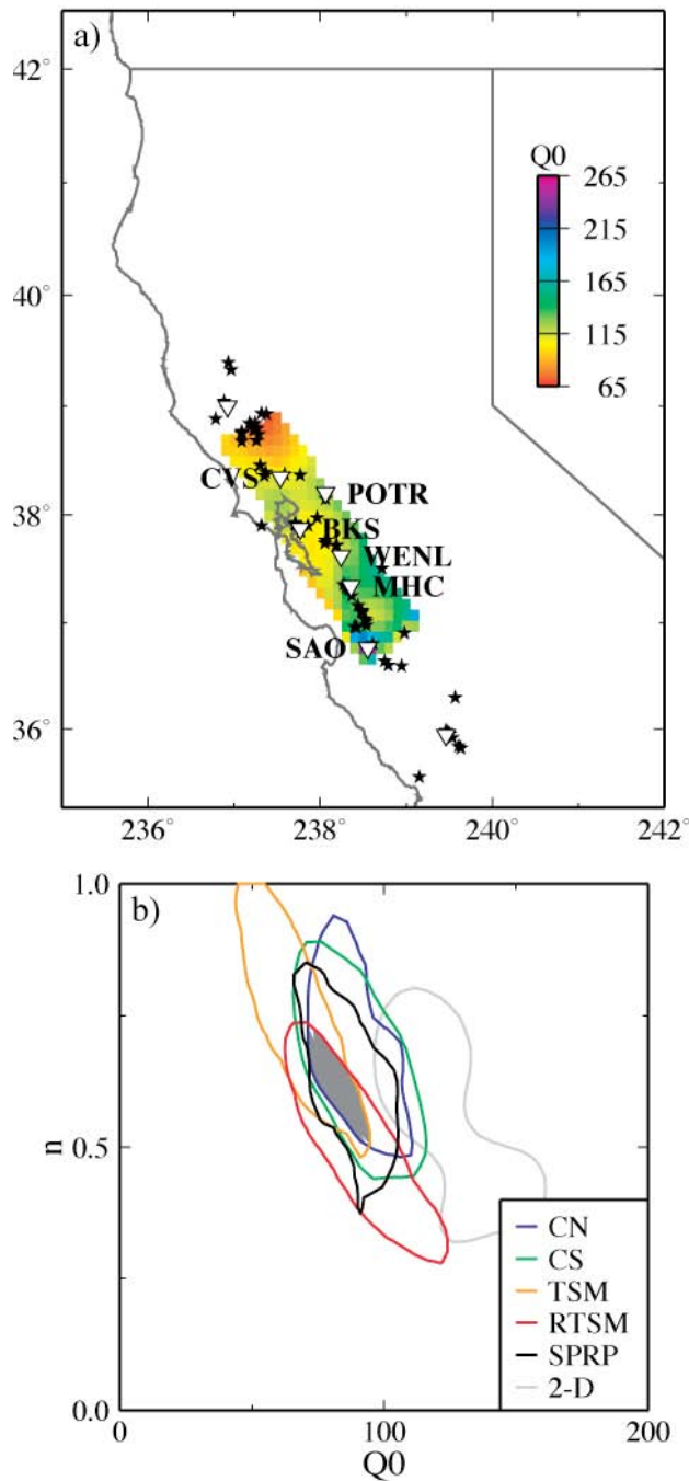
Figure 3. Method comparison with tomographic results of (Mayeda et al. 2005). (a) Region where 2-D direct wave attenuation coefficients are used, which covers the same area as the paths and stations in Figure 2a. (b) Comparison of tomographic results where empirical distribution (light grey) is from data at each node with 1-D results.
