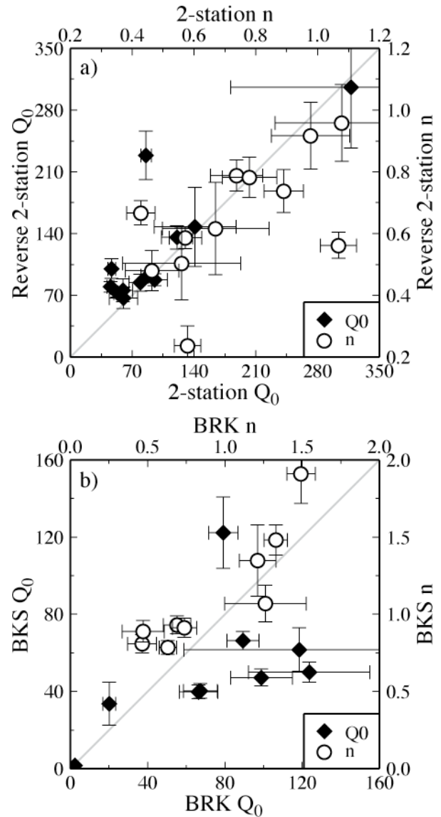
Figure 6. An investigation into site effects. (a) Power-law parameters for paths measured by both the RTS and TS methods. (b) Power-law parameters measured at nearly co-located stations BKS and BRK using the TS method.
