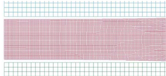
Figure 6. Mesh plot at 286 \mu\text{s} for the linear elastic specimen with a Poisson's ratio of 0.49900, a Young's modulus of 430 kPa and for t_R = 25 \mu\text{s} . The centerline is on the left and the incident bar is at the bottom.
