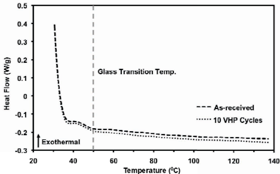
Figure 32: DSC Diagram of the Insulation Layer on the Aviation Wire
