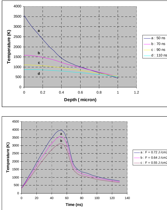
Figure 10(b) Calculated temperature at various depths of the irradiated surface after different time of the initiation of the pulse.
