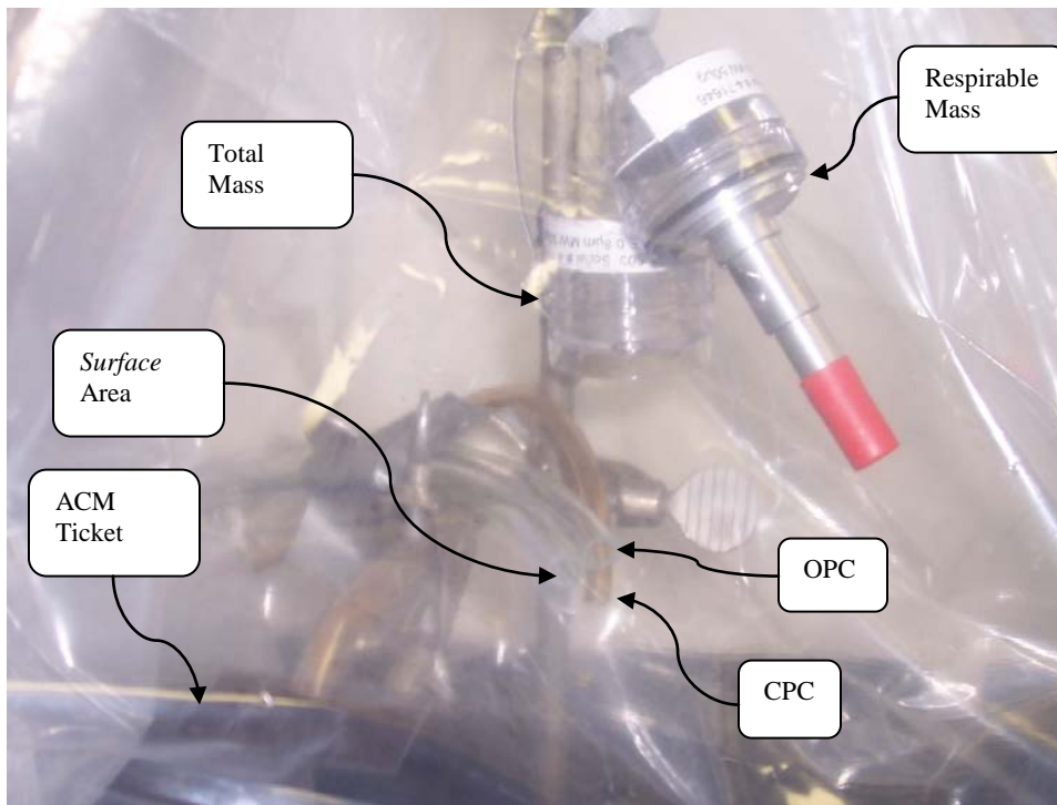
Figure 6 Sampling setup
