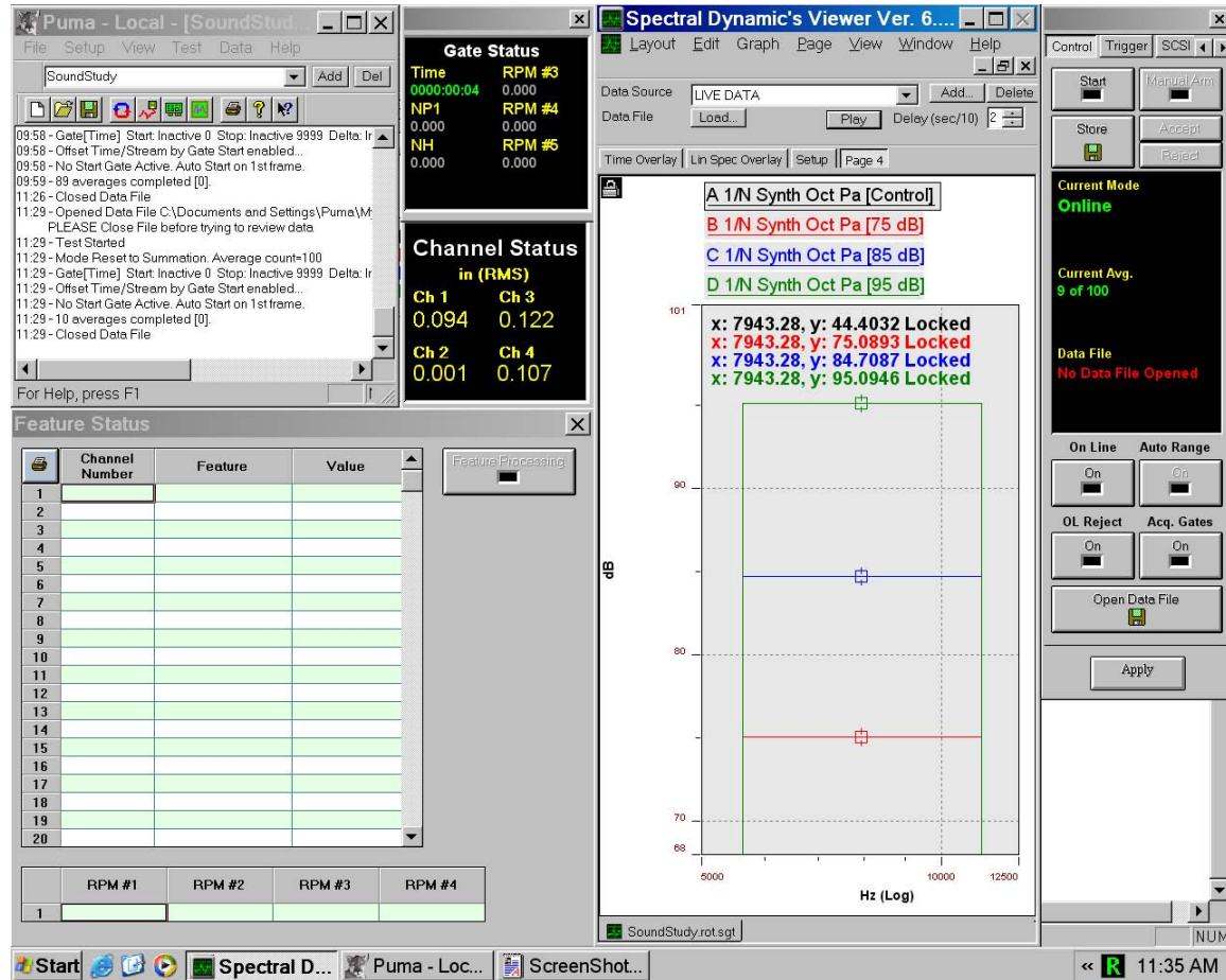
Figure 27. Screen capture of Puma data acquisition system
