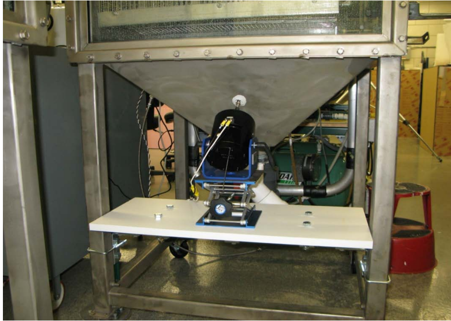
Figure 8. Shaker mounted on shelf between chamber legs
