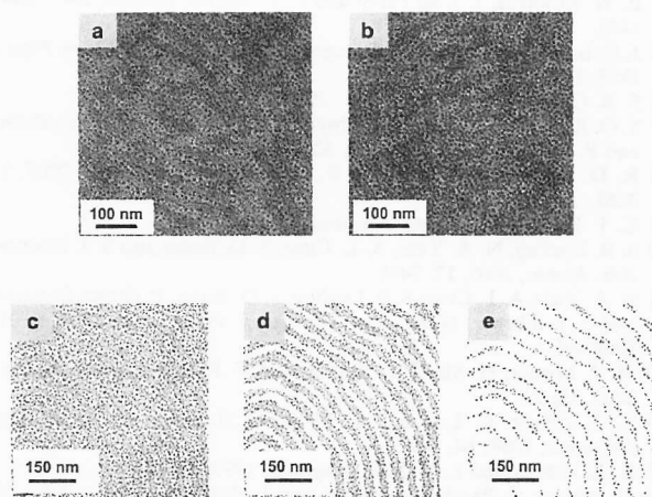
Fig. 3 Au-coated PS- b -PMMA films, as seen under TEM. There is little difference between pristine (a) and UV-irradiated (b) samples, suggesting that gold particles remain upon PMMA removal. (c)–(e) A pristine gold-coated PS- b -PMMA sample with (c) all of the gold particles, (d) particles on PMMA domains removed by hand, and (e) particles on PS removed.
