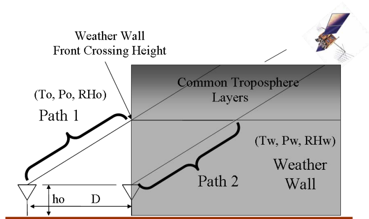
Fig. 10. Troposphere Model for Worst Case Spatial Decorrelation.
