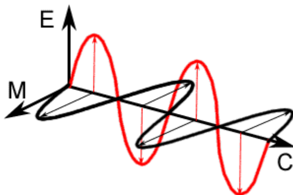
Exhibit C-3. Electromagnetic Wave
