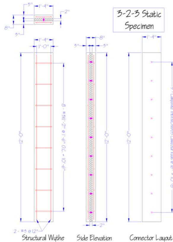
Figure 5. Conventionally Reinforced 3-2-3 Static Sandwich Panel Specimen
