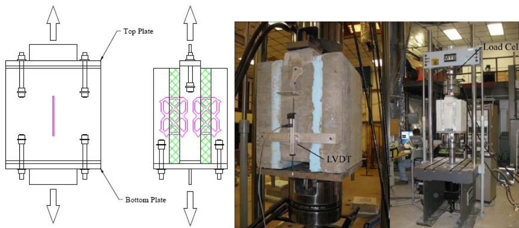
Figure 6. Shear Tie Static Test Configuration
