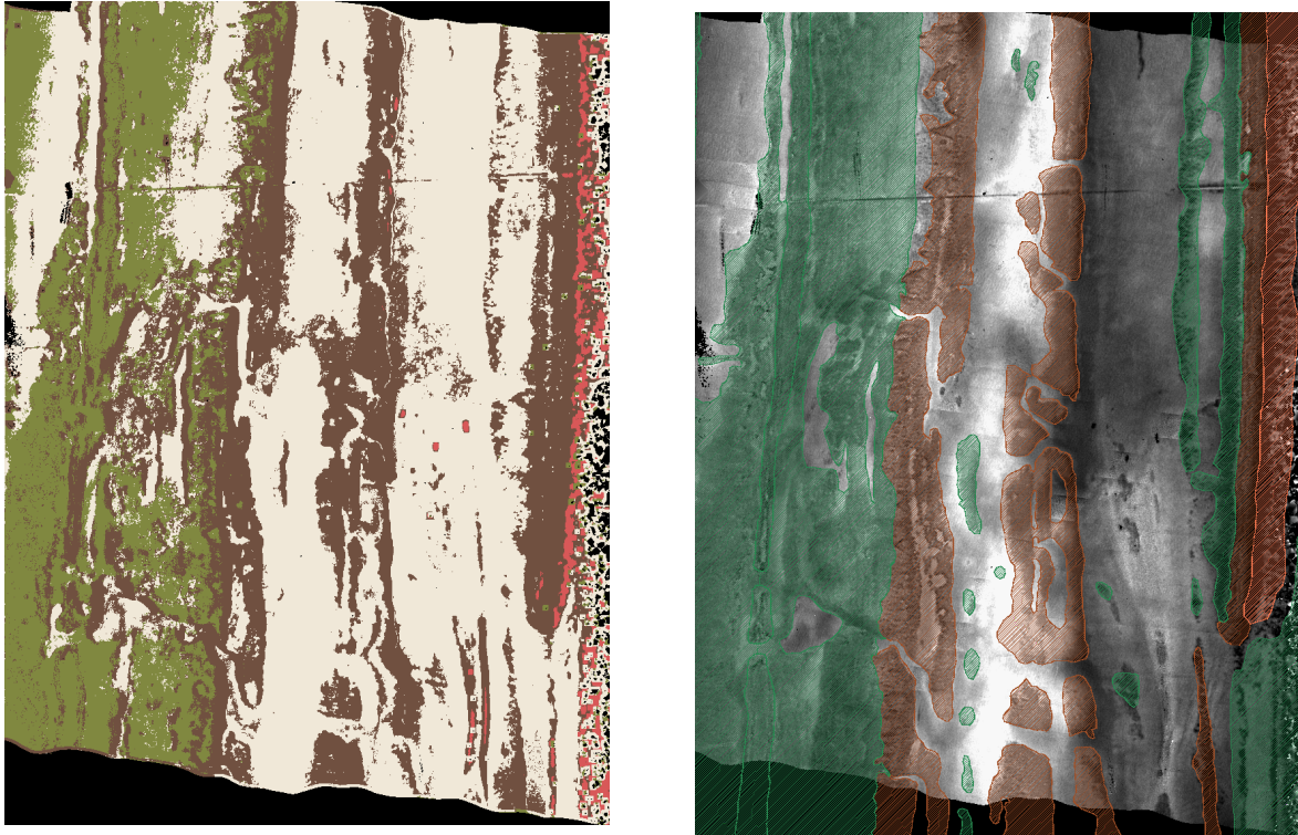
Figure 3. SHOALS seafloor classification (left) of South Block dataset, and ground truth (overlaid on seafloor reflectance image) right.
