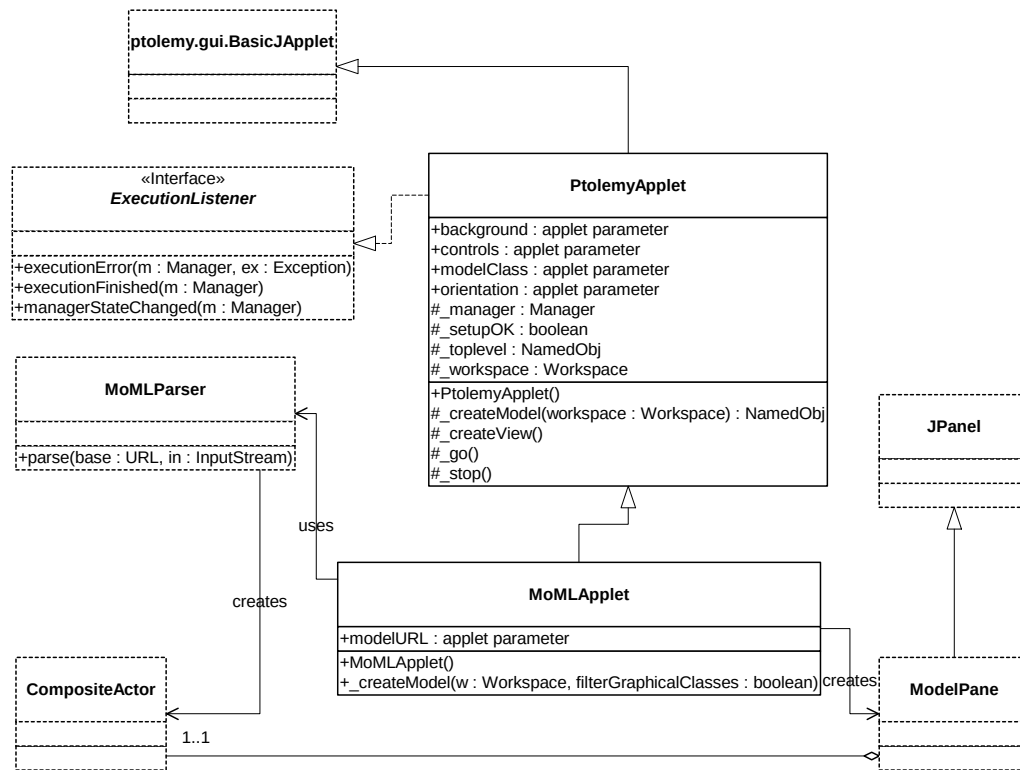
FIGURE 8.1. UML static structure diagram for PtolemyApplet, a convenience class for constructing applets. PtolemyApplet is in the ptolemy.actor.gui package.
