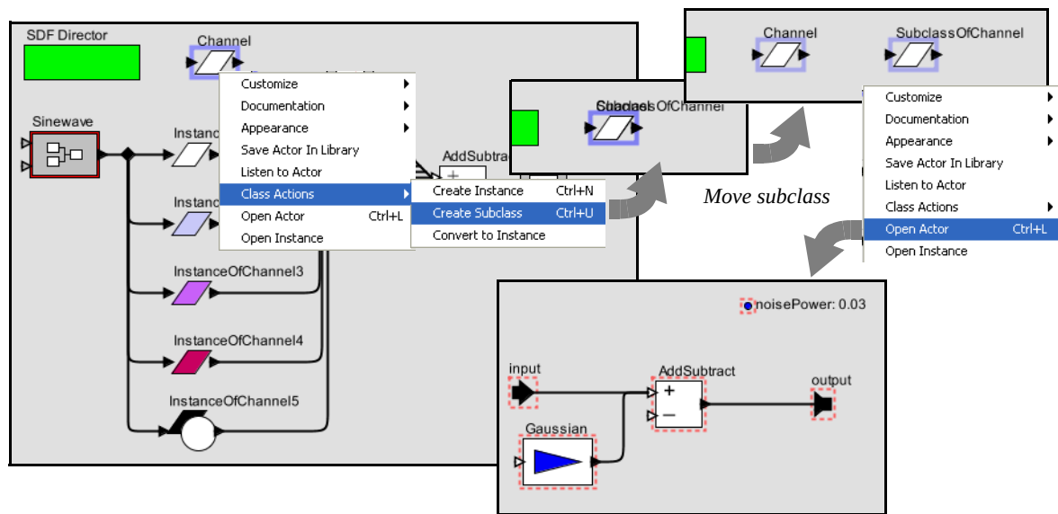
FIGURE 2.39. The model from figure 2.38 with a subclass of the Channel with no overrides (yet).
