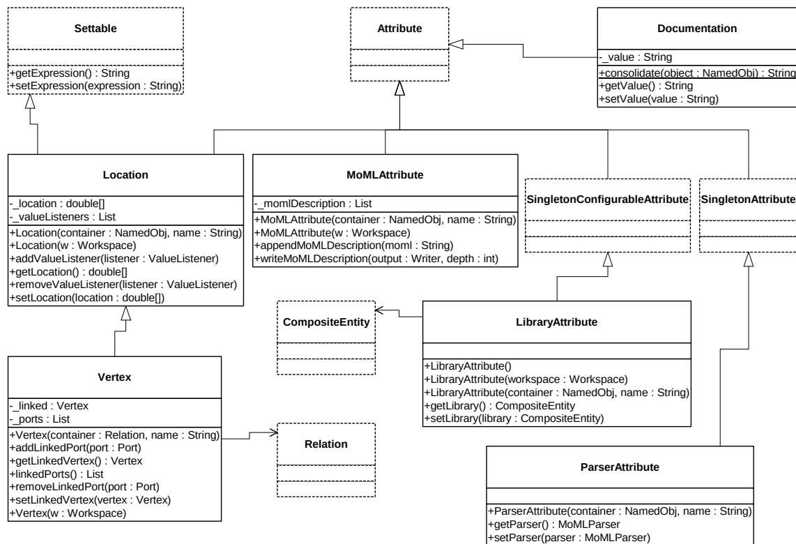
FIGURE 7.11. Attributes in the moml package.
