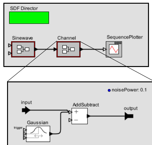
FIGURE 2.34. Hierarchical model that we will modify to use classes.
