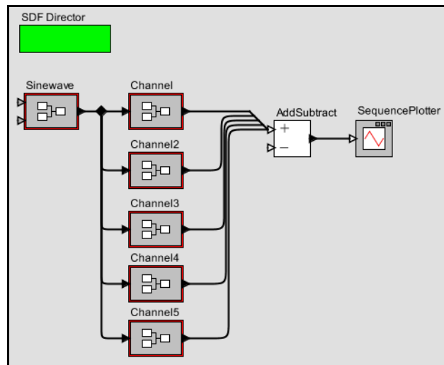
FIGURE 2.35. A poor design of a diversity communication system, which has multiple copies of the channel as defined in figure 2.34.
