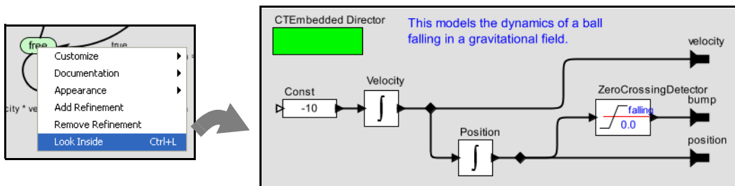
FIGURE 2.60. The refinement of the free state, shown here, is a continuous-model representing the laws of gravity.
