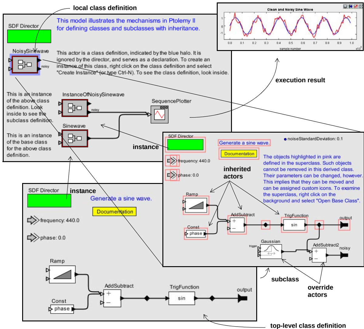
FIGURE 1.4. Illustration of actor-oriented classes, subclasses, and inheritance.
