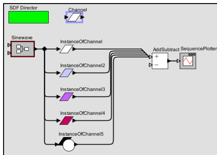
FIGURE 2.38. The model from figure 2.37 with the icons of the instance changed to override parameter values in the class.
