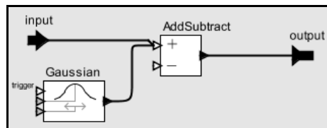
FIGURE 2.24. A simple channel model defined as a composite actor.
