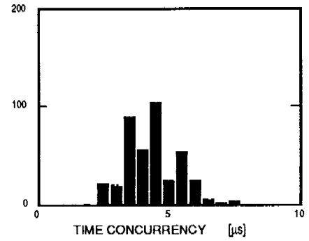
Fig. 5 Time concurrency distribution in stage 2
