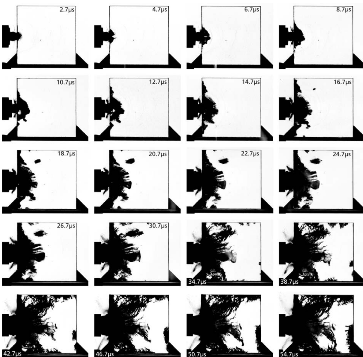
Figure A-3. Complete set of high-speed photographs from baseline test with Starphire, spherical projectile, impact velocity 432 m/s, test no. 16595.
