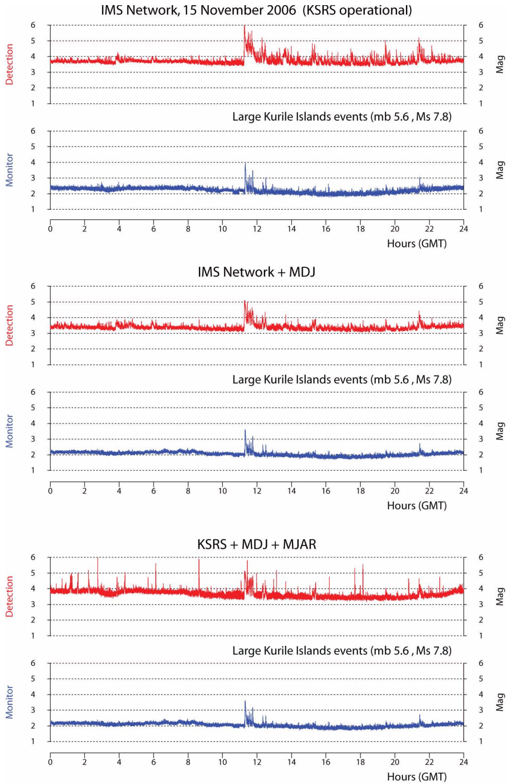
Figure 6. This figure shows a one-day plot of detection traces (red) and monitoring traces (blue) for 15 November 2006. The top panel uses IMS stations (including KRSR); the middle panel shows the effect of adding the MDJ station and the bottom panel shows results from using only KRSR, MDJ and MJAR.
