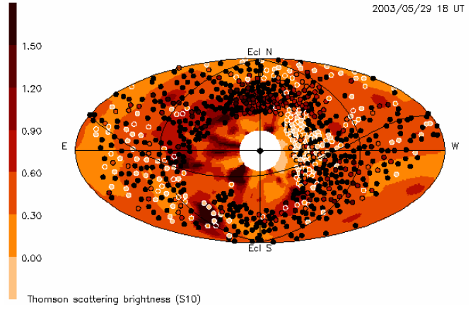
Figure 7. SMEI image depicting all of the sky as observed from Earth and including the positions of the edited lines of sight present within a day of the indicated time. The data point color indicates the relationship of the line-of-sight brightness signal at these locations relative to the brightness in the Thomson scattering reconstruction.
