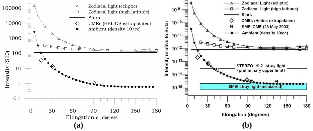
Figure 3. Surface brightness versus solar elongation for zodiacal and starlight (Allen's Astrophysical Quantities , 2000), and of expected CME brightness extrapolated from Helios measurements. A calculation of an ambient medium having a density of 10 \text{ e}^- \text{ cm}^{-3} at 1 AU and an inverse-square density dropoff with solar distance is also shown. a) Brightness in S10, (Figure 2) at 1 AU. b) Brightness relative to sunlight at 1 AU. Also shown is the brightness of a large SMEI-observed CME, and the stray light levels observed in SMEI, and also that reported from the STEREO HI-2 instruments.
