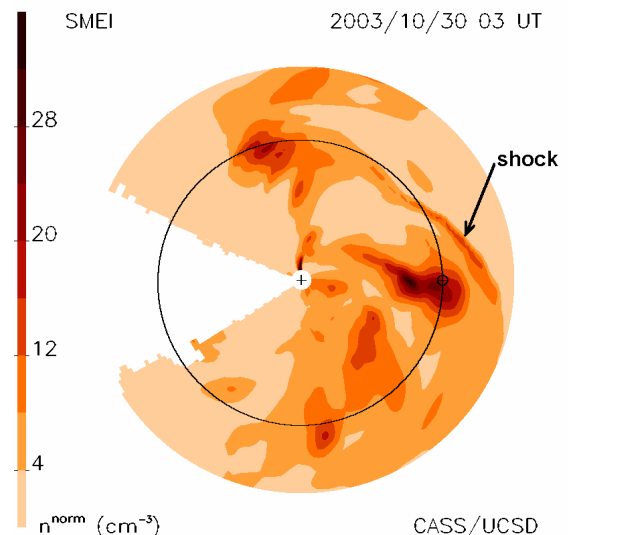
Fig. 11. SMEI-derived density ecliptic cut showing the 3D reconstruction of the density enhancement behind a shock.
