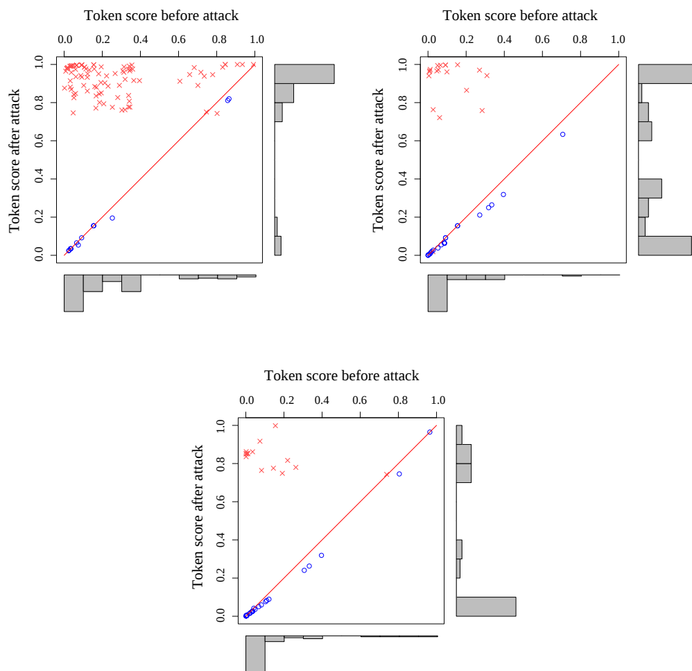
Figure 2: Effect of the focused attack on three representative emails. Each point is a token. The x-axis is the token spam score before the attack (0 means ham and 1 means spam); the y-axis is the spam score after the attack. The red \times 's are tokens included in the attack and the blue \circ 's are tokens that were not in the attack. Histograms show the distribution of token scores before the attack (at bottom) and after the attack (at right).
