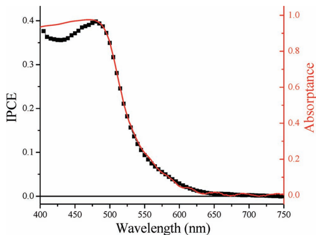
Figure 3. IPCE and absorbance spectrum of a Ru(deeb) 2 (BTL)/TiO 2 thin film. The photocurrent action spectrum was measured in 0.50 M LiI and 0.50 M I 2 /acetonitrile, while the absorbance spectrum was measured in 0.1 M LiClO 4 /acetonitrile.
