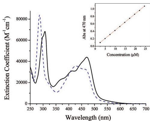
Figure 1. Absorption spectra of \text{Ru}(\text{deeb})_2(\text{BTL})(\text{PF}_6)_2 (solid line) and \text{Ru}(\text{bpy})_2(\text{BTL})(\text{PF}_6)_2 (dashed line) in neat acetonitrile. The inset shows the concentration dependence of the \text{Ru}(\text{deeb})_2(\text{BTL})(\text{PF}_6)_2 absorbance at 470 nm. The best-fit line yielded an extinction coefficient of 44\,300\text{ M}^{-1}\text{ cm}^{-1} .
