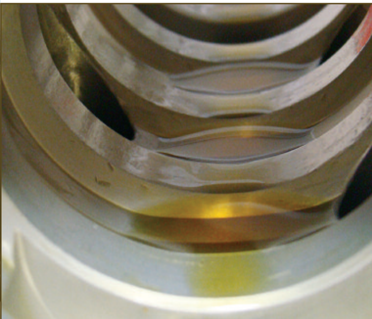
Left: Internal view of the valve body. Photos courtesy of Erin Murcko, NSWCCD-SSS Division.
