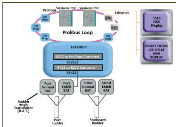
Pre-November 2006 Rudder Design.
