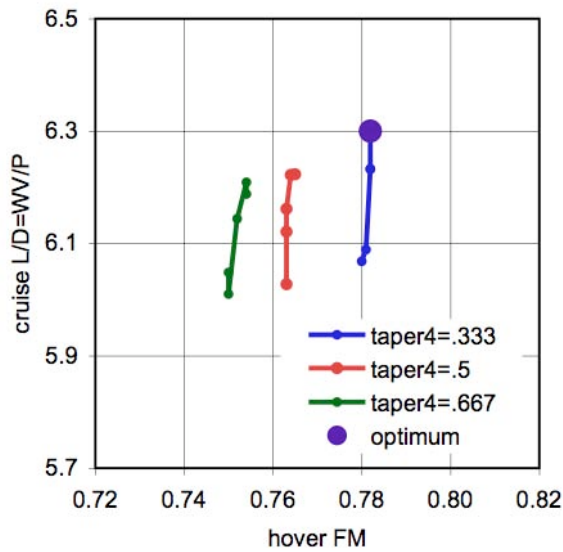
Figure 48. Effect of taper on lift-offset coaxial helicopter performance (taper = tip/root chord ratio). Inboard taper fixed at 1.333 ; taper3 extends from 0.5R to 0.75R , taper4 from 0.75R to 1.0R . For each taper4 value, taper3 varies from 0.667 to 1.5 .
