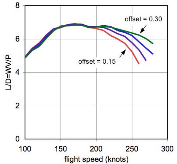
Figure 50. Lift-offset coaxial helicopter aircraft lift-to-drag ratio, L/D = WW/P (offset = 0.15 , 0.20 , 0.25 [design], 0.30 ).
