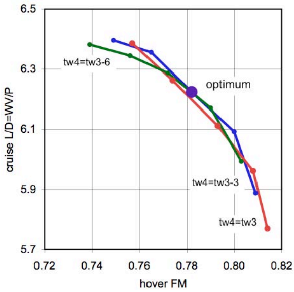
Figure 47. Effect of twist on lift-offset coaxial helicopter performance (twist = linear rate, root to tip). Inboard twist fixed at -3/-6 deg; tw3 extends from 0.5R to 0.75R , tw4 from 0.75R to 1.0R . For each curve, tw4 varies from -12 to -24 deg.
