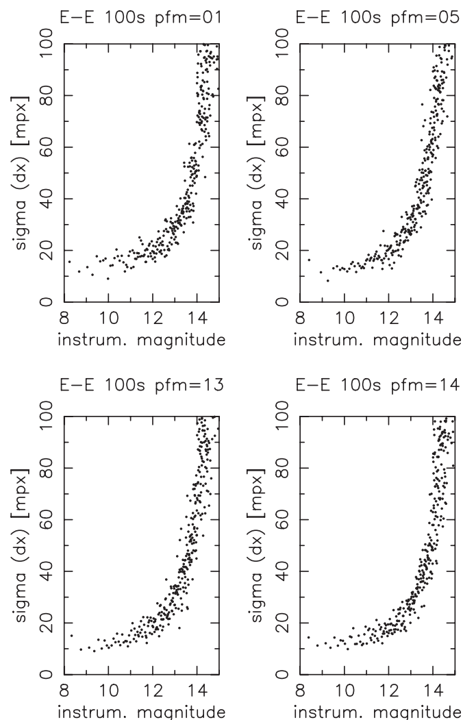
Figure 9. Standard error (sigma) of the x-coordinate as a function of instrumental model magnitude from the comparison of two 100 s exposures taken of the same field in the sky within minutes. Results are shown from the same CCD frame pair but for different image profile fit models (pfm) as indicated. The error shown is the combined error of both exposures, dominated by atmospheric effects. Each dot represents the rms average of 16 stars. Unit is millipixel (1 mpx = 0.9 mas).
