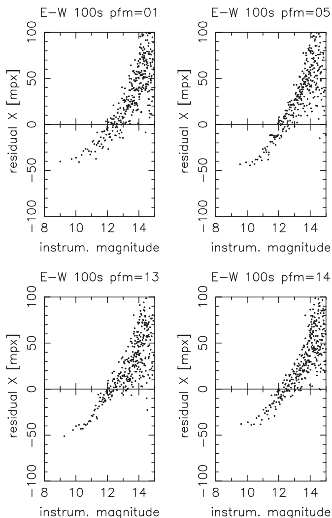
Figure 10. Systematic differences between the x-coordinates of a pair of 100 s exposures taken from opposite sides of the telescope pier (rotated by 180^\circ with respect to each other) as a function of instrumental model magnitude, after a linear transformation of the x, y data but without any other corrections applied. Results are shown from the same CCD frame pair but for different image profile fit models (pfm) as indicated. Each dot represents the mean over 16 stars. Unit is millipixel (1 mpx = 0.9 mas).
