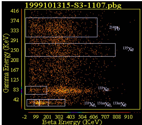
Figure 1. Two-dimensional beta/gamma spectrum (taken from McIntyre et al., 2006).
