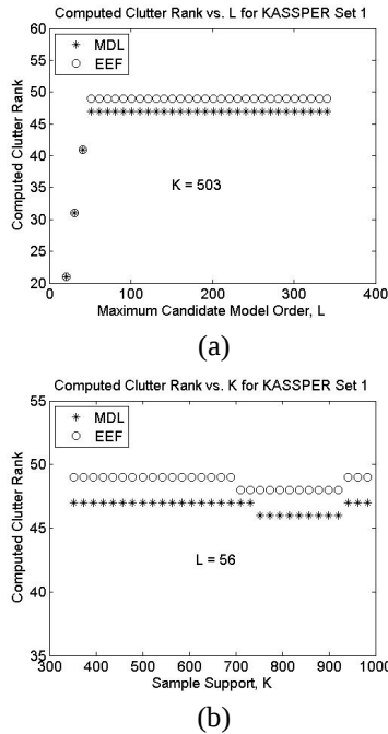
Fig. 3. Computed clutter ranks using EEF and MDL estimators for set 1 as functions of (a) L and (b) K
