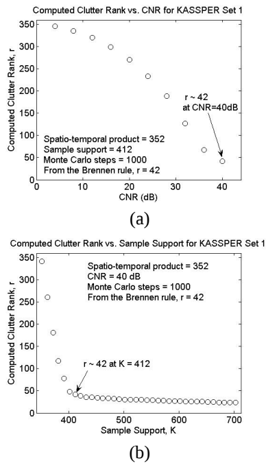
Fig. 5. Computed clutter ranks using CWA method for set 1 as functions of (a) CNR and (b) K
