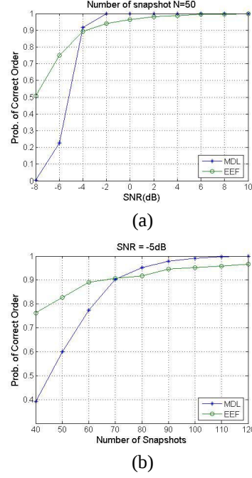
Fig. 2. Probabilities of correct order for EEF and MDL as functions of (a) SNR ( p = 7 , N = 50 ) and (b) Number of Snapshots ( p = 7 , SNR = -5 dB)
