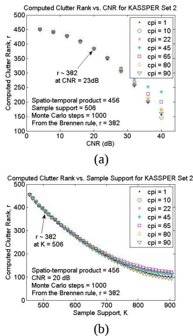
Fig. 6. Computed clutter ranks using CWA method for set 2 as functions of (a) CNR and (b) K
