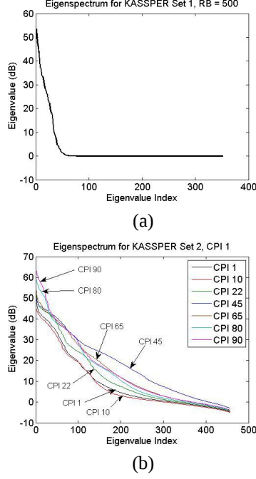
Fig. 1. Eigenspectra of the clutter-only (a) set 1 and (b) set 2
