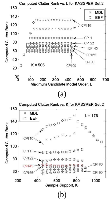
Fig. 4. Computed clutter ranks using EEF and MDL estimators for set 2 as functions of (a) L and (b) K
