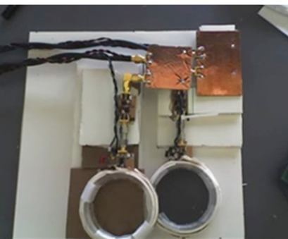
Above: A Tursiop 4-channel coil built as 2 pairs of loops, with each pair placed on either side of an object to be imaged. Left: Early proof of concept, a brain at 0.24mm resolution.
