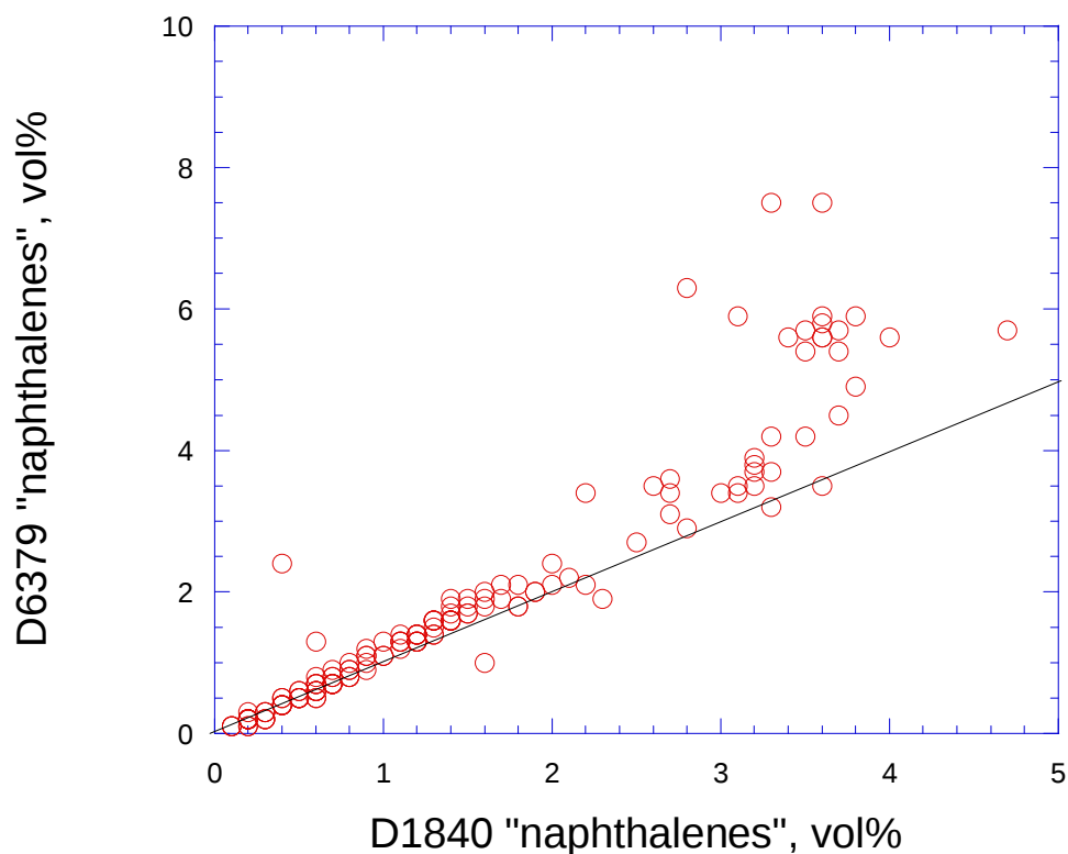
Figure11. Correlation between total naphthalenes by ASTM D1840 and D6379.
