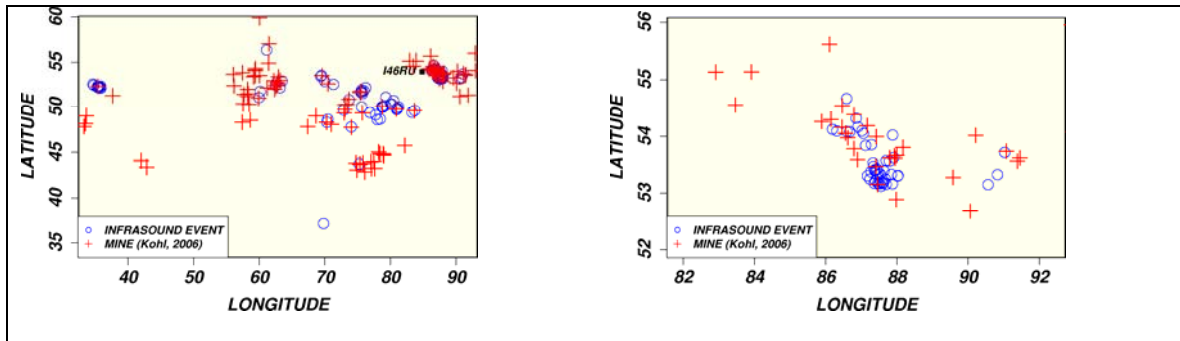
Figure 7. The left plot shows mines (red crosses) in Eurasia compiled by Kohl (2006) together with events (blue circles) with associated infrasound signals recorded at the IMS station Zalesovo (I46RU) indicated in upper right. The events occurred between January and June of 2007. The large number of mines just to the east of the station is in the Kuzbass mining district. The plot to the right shows mines and events with infrasound signals in the Kuzbass district and surrounding areas. Most of the Kuzbass events were located near two mines in the extreme southern part of the district.
