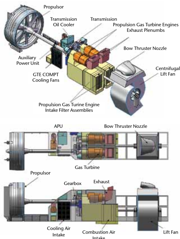
Above: Drawing showing the equipment arrangement for the SSC's power plant and propulsor. SSCs are similar to LCACs regarding air cushion vehicle technology.
