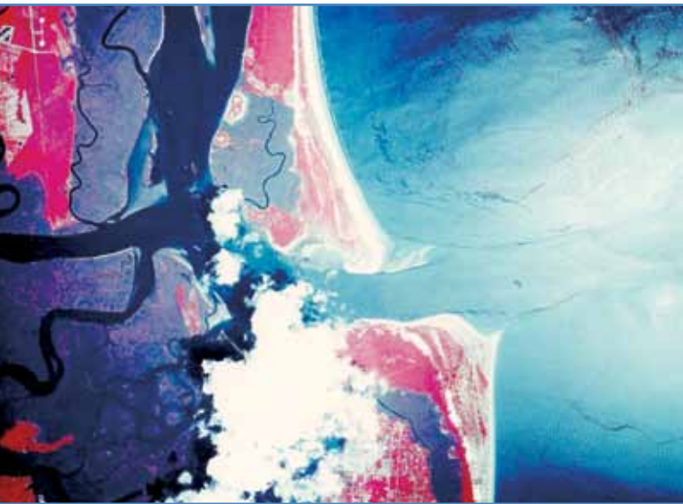
Left: An aerial view of the channel approach to Kings Bay. The channel is in the center and right center, and is about 11 miles in length. EMOGS uses wave measuring buoys and measured tide levels to assist harbor personnel in figuring whether the channel can permit the safe passage of ships.
