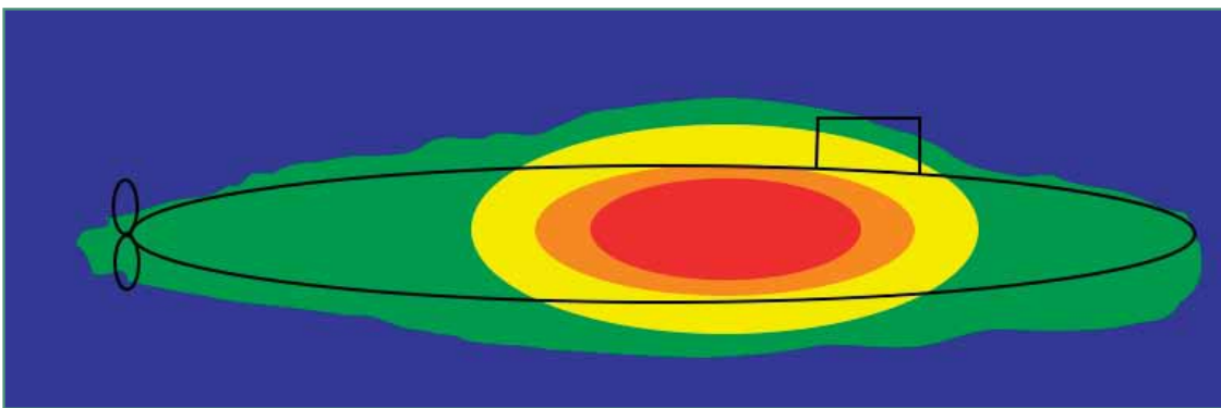
Left: Colors delineate a typical area of acoustic intensity detected with accuracy by spotbeams. Image courtesy of Mike Marsh, NSWC Carderock Division..
