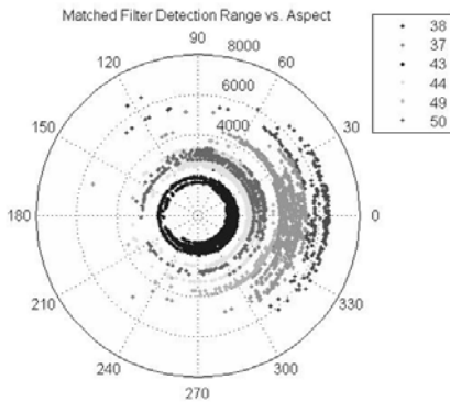
Figure 15: Detection range vs. aspect from the tagged whale's head: Matched filter detector
