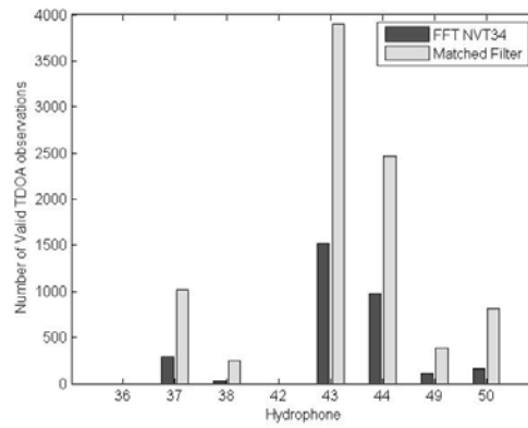
Figure 9: Detection efficacy per hydrophone
