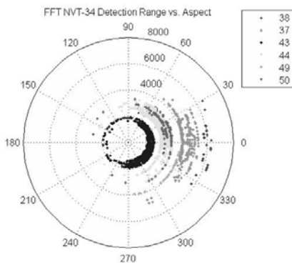
Figure 14: Detection range vs. aspect from the whale's head: FFT (NVT34) Detector
