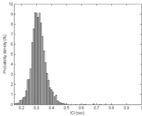
Figure 8: Probability density function for foraging click ICIs
