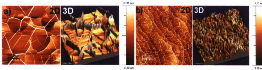
Figure 9. AFM images show the improvement in C face graphene achieved during our study. Image (a) shows the extent of the folds in a relatively thick graphene layer on the carbon face estimated to be about 25 to 30 monolayers. Image (b) is carbon face graphene that's about 5 to 8 monolayers thick.
