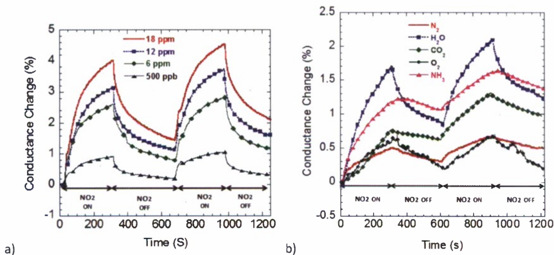
Figure 11: a) The change of conductance of graphene formed on the C-face of SiC for various amounts of NO 2 . b) The change of conductance in epitaxial graphene layers grown on (a) Si- face, and (b) C-face of SiC for different concentrations of N 2 , NH 3 , CO 2 , O 2 , and H 2 O
