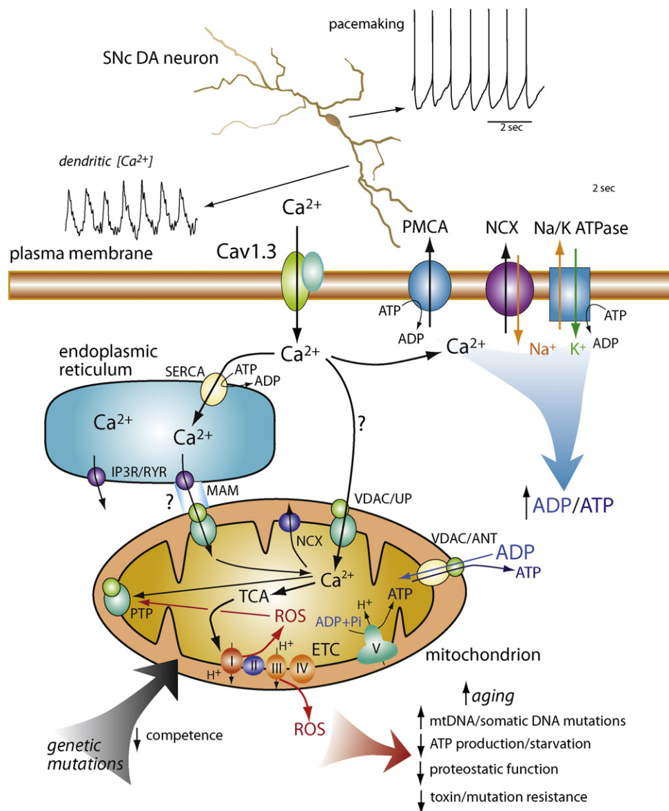
Fig. 2. A schematic summarizing a model of how \text{Ca}^{2+} entry during pacemaking in SNc DA neurons might lead to mitochondrial oxidative stress, accelerated aging and eventual cell death. At the top is an image of a reconstructed SNc DA neuron showing the pacemaker driven somatic spiking and dendritic \text{Ca}^{2+} oscillations associated with pacemaking. This dendritic \text{Ca}^{2+} influx is attributable almost entirely to flux through Cav1.3 \text{Ca}^{2+} channels. At the bottom is a cartoon depicting the hypothetical mechanisms involved in elevating mitochondrial oxidative stress. \text{Ca}^{2+} influx through Cav1.3 channels is either sequestered in the endoplasmic reticulum by uptake through smooth endoplasmic reticulum \text{Ca}^{2+} (SERCA) pumps or taken up by mitochondria through channels created by voltage-dependent anion channels (VDAC) and \text{Ca}^{2+} uniporter (UP); the extent to which this pathway is important is in question (hence the question mark on the arrow). \text{Ca}^{2+} could also enter mitochondria through this VDAC/UP channel at points of apposition between the ER and mitochondria where inositol trisphosphate receptors (IP3) and/or ryanodine receptors (IP3R/RyR) are positioned at specializations – mitochondrial associated membrane (MAM). This entry route has not been established in SNc DA neurons, hence the question mark. \text{Ca}^{2+} entering through Cav1.3 channels is moved back across the plasma membrane through either the \text{Ca}^{2+} -ATPase (PMCA) or through a \text{Na}^{+}/\text{Ca}^{2+} exchanger (NCX) that relies upon the \text{Na}^{+} gradient maintained by the Na/K ATPase at energetic cost; leading to conversion of ATP to ADP. ADP and ATP are exchanged by mitochondria with the VDAC and adenine nucleotide transporter (ANT). ADP stimulates oxidative phosphorylation. \text{Ca}^{2+} entering the mitochondrial matrix can stimulate enzymes of the tricarboxylic acid (TCA) cycle that produces reducing equivalents for the electron transport chain (ETC); complex I through V are shown at the inner mitochondrial membrane; complex V (ATP synthase) uses the electrochemical gradient to convert adenosine diphosphate (ADP) and inorganic phosphate to adenosine triphosphate (ATP). Electron movement along the ETC generates superoxide, leading to the production of reactive oxygen species (ROS) that can produce a variety of deleterious effects that can be viewed as accelerated aging (red arrow at the bottom). One other action of ROS is to promote opening of the mitochondrial permeability transition pore (mPTP); irreversible opening of the mPTP leads to release of pro-apoptotic factors into the cytosol. A basic question is whether reversible opening of the mPTP is possible under conditions of mild oxidative stress; mPTP opening and depolarization of the inner mitochondrial membrane could serve to diminish ROS production. \text{Ca}^{2+} is removed from mitochondria through mitochondrial \text{Na}^{+}/\text{Ca}^{2+} exchangers (NCXs). Lastly, genetic mutations associated with Parkinson's disease, like those to DJ-1 or PINK1, might directly compromise the competence of mitochondria, leading to accelerated aging or increased oxidative stress.
