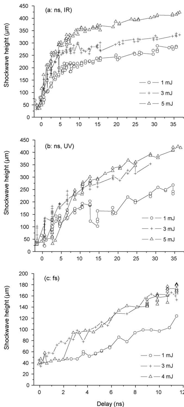
Fig. 4. Heights of shockwaves associated to the plasmas induced on the surface of a nylon sample by nanosecond IR (1064 nm, a), UV (266 nm, b), and femtosecond IR (800 nm, c) laser pulses, with pulse energies of 1, 3 and 5 mJ for the case of nanosecond pulses, and 1, 3 and 4 mJ for the case of femtosecond pulses.
