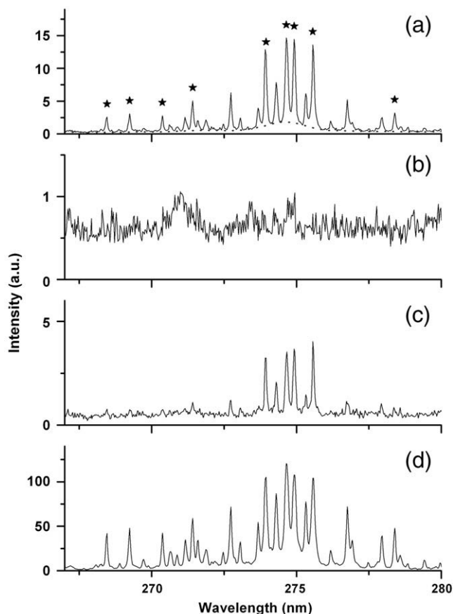
Fig. 3. LIBS spectra of iron from a) a single Nd:YAG pulse, b) a single \text{CO}_2 laser pulse, c) double pulse spectra with \text{CO}_2 following Nd:YAG by 1 \mu\text{s} compared with Nd:YAG alone LIBS spectrum and d) double pulse spectra with \text{CO}_2 preceding Nd:YAG by 1 \mu\text{s} . (Acquisition delay: 1 \mu\text{s} , duration of acquisition: 25 ns). In a), the dotted line shows a background spline interpolation and the stars indicate the lines used for plasma temperature calculation. Baseline correction is applied for all spectra.
