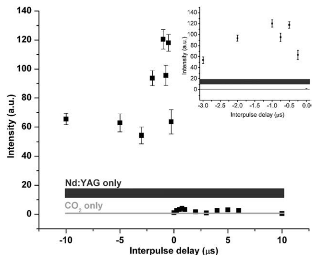
Fig. 4. Background-corrected peak intensity of the Fe II 274.65 nm line as a function of the interpulse delay. A negative delay means the \text{CO}_2 pulse reaches the samples before the Nd:YAG pulse. A positive delay is for the opposite timing configuration. Comparison is made with the single-pulse cases. The error bars represent the standard deviation over 30 single acquisitions. The inset in the upper right corner is a zoom between -3 \mu\text{s} and 0 \mu\text{s} showing the maximum enhancement at -1 \mu\text{s} .
