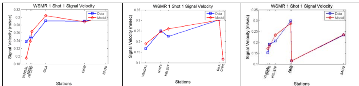
Figure 11. Variation of signal group velocity in recorded and modeled waveforms with source-receiver distance.
