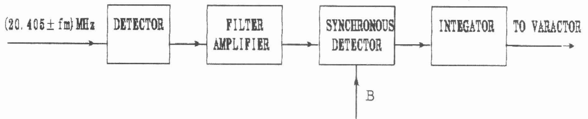
Fig. 8. Lock-in Amplifier
