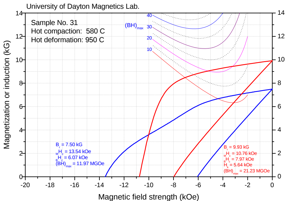
Figure 11. Demagnetization curves of specimen No. 31, \text{Pr}_{14.1}\text{Fe}_{73.3}\text{Co}_{5.1}\text{Ga}_{0.5}\text{B}_{7.1} / \text{Pr}(\text{Co}_{0.8}\text{Fe}_{0.2})_5 (80 wt%/20 wt%), after hot compaction at 580°C and hot deformation at 950°C.
