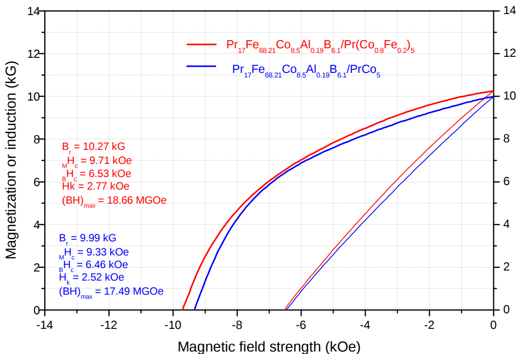
Figure 24. Demagnetization curves of \text{Pr}_{17}\text{Fe}_{68.21}\text{Co}_{8.5}\text{Al}_{0.19}\text{B}_{6.1}/\text{PrCo}_5 and \text{Pr}_{17}\text{Fe}_{68.21}\text{Co}_{8.5}\text{Al}_{0.19}\text{B}_{6.1}/\text{Pr}(\text{Co}_{0.8}\text{Fe}_{0.2})_5 magnets.
