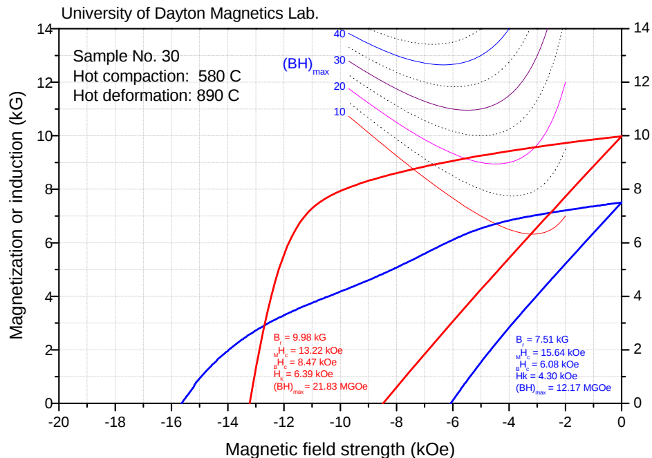
Figure 10. Demagnetization curves of specimen No. 30, \text{Pr}_{14.1}\text{Fe}_{73.3}\text{Co}_{5.1}\text{Ga}_{0.5}\text{B}_{7.1} / \text{Pr}(\text{Co}_{0.8}\text{Fe}_{0.2})_5 (80 wt%/20 wt%), after hot compaction at 580°C and hot deformation at 890°C.
