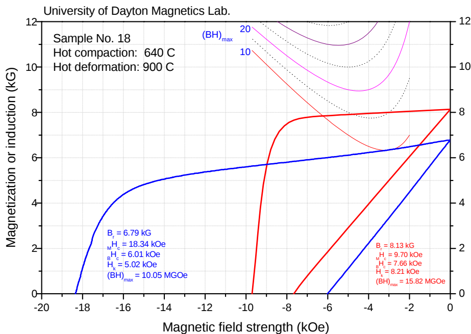
Figure 3. Demagnetization curves of \text{PrCo}_5 specimen No. 18 after hot compaction at 640°C and hot deformation at 900°C.
