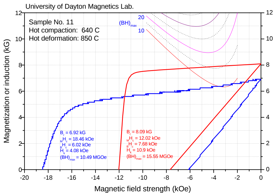
Figure 2. Demagnetization curves of \text{PrCo}_5 specimen No. 11 after hot compaction at 640°C and hot deformation at 850°C.
