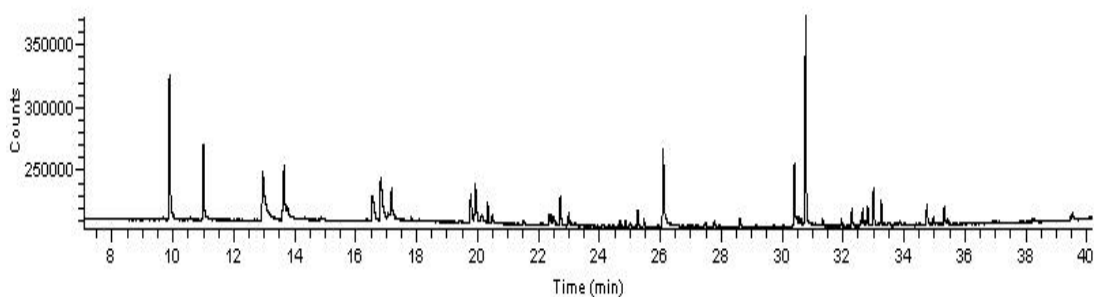
Figure 6.3: Chromatogram of the 700 K n-decane oxidation sample.
