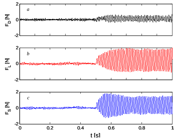
Figure 4.18 Time traces of the relative measured drag (a), lift (b), and side (c) forces, for the flow actuated by modulation of the top and left jet at 100 Hz.
