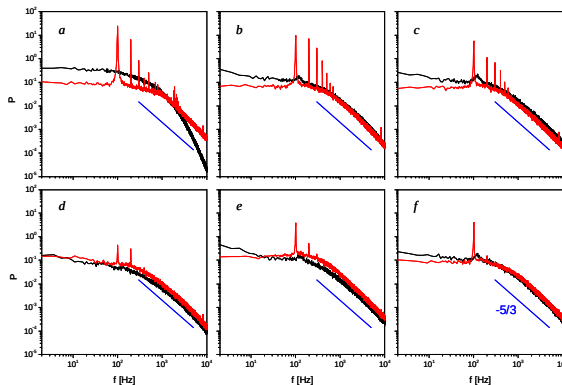
Figure 4.20 Power spectra of the velocity fluctuations at the upper shear layer (a-c) and the wake core (d-f) for the baseline (—) and the flow actuated by both continuous top and left jets modulated at 100 Hz (—) at x/R = 0.55 (a, d), 1.5 (b, e), and 2.45 (c, f).
