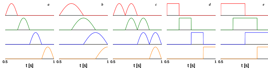
Figure 4.23 Schematics of the spinning actuation cycles depicting sequential activation of the top (—), right (—), bottom (—) and left (—) jets in: sinusoidal (a), overlapping sinusoidal (b), double sinusoidal (c), square (d), and overlapping square patterns (e).
