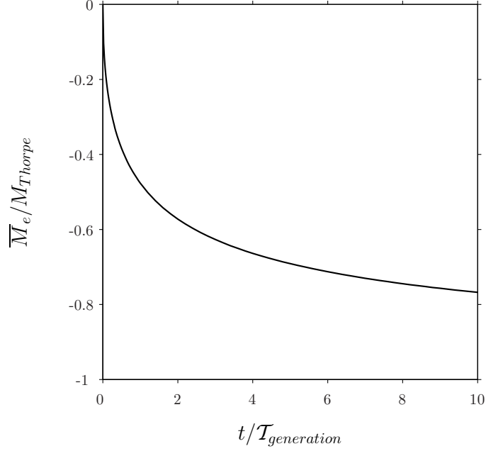
Figure 2-4: The analytical solution for the upslope Ekman transport scales with M_{T\text{horpe}} = \kappa/\theta and evolves in time on the buoyancy generation timescale.
