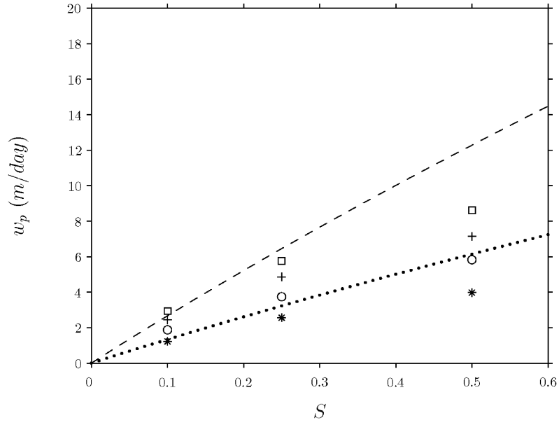
Figure 4-6: The average Ekman pumping, w_p , calculated from t/\mathcal{T}_{inertial} = 1.0 - 4.0 , is shown with respect to S from the \theta = 0.01 runs. The symbols correspond to U = 5 \text{ cm s}^{-1} (*), U = 10 \text{ cm s}^{-1} (o), U = 15 \text{ cm s}^{-1} (+), U = 20 \text{ cm s}^{-1} (□). The dashed line indicates the estimated w_{upwelling} as a function of S from the initial flow parameters, where U_{slope} = U_{shelf} = U , and the dotted line corresponds to w_{upwelling} , where U_{slope}/U_{shelf} = 2 .
